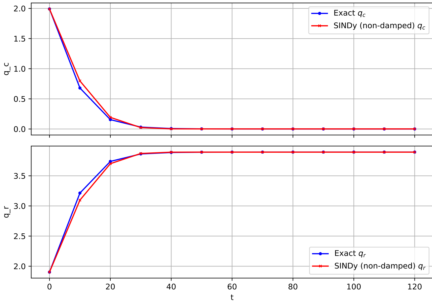
Trajectory 1291 (non-damped)
