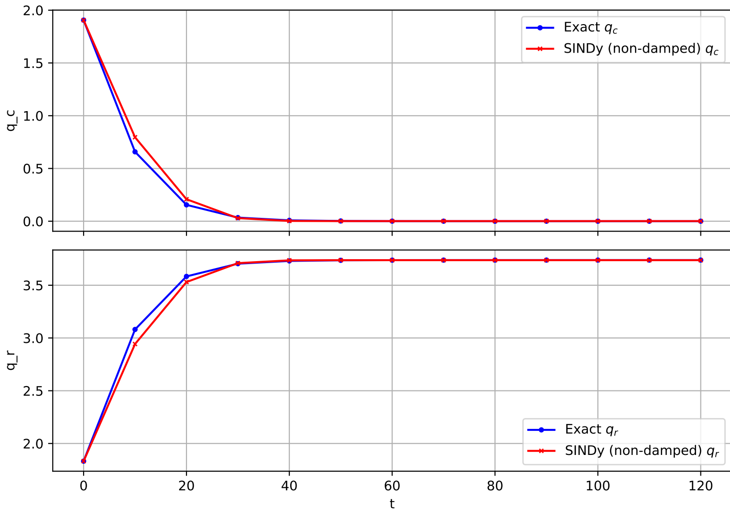
Trajectory 1292 (non-damped)
