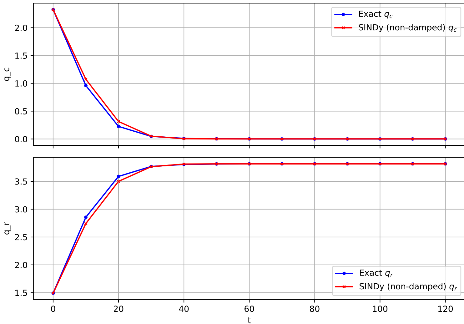
Trajectory 1299 (non-damped)
