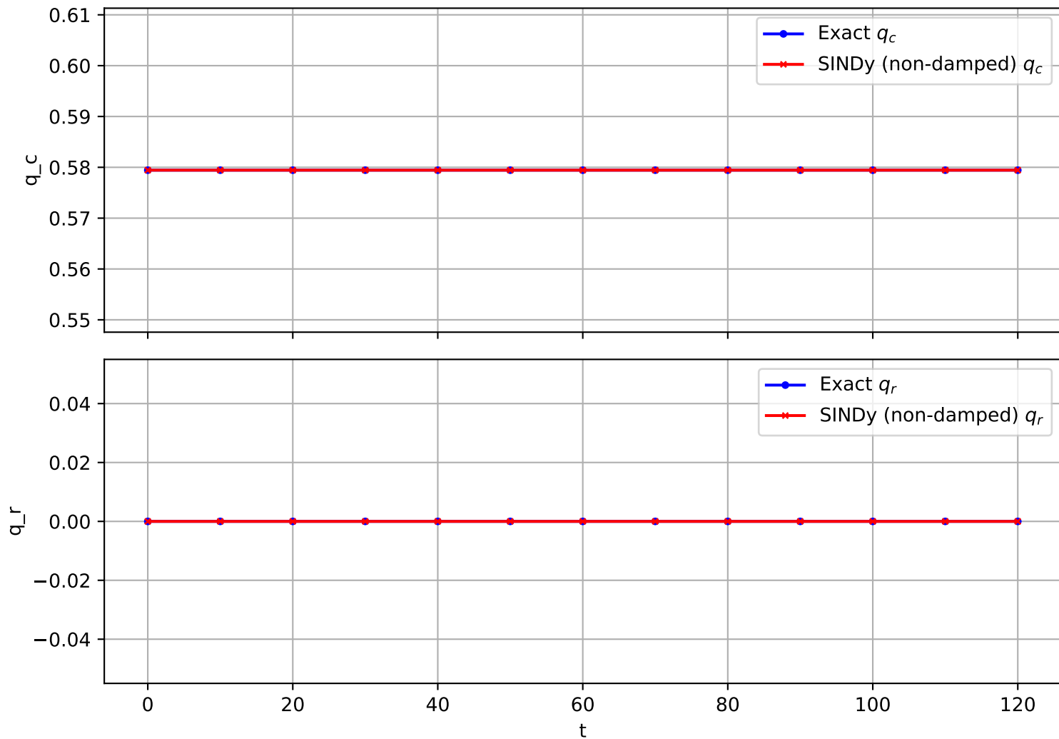
Trajectory 13 (non-damped)
