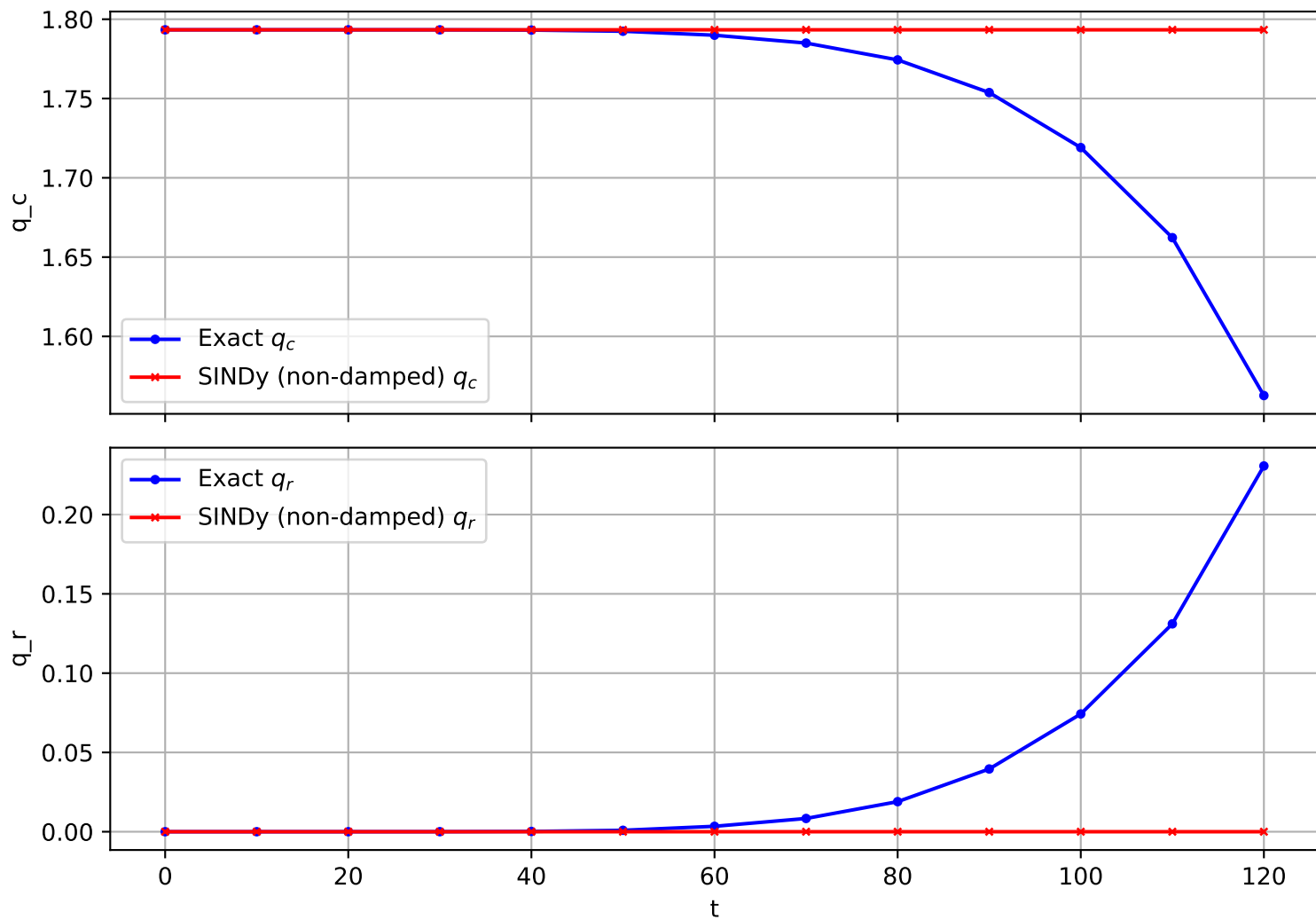
Trajectory 130 (non-damped)
