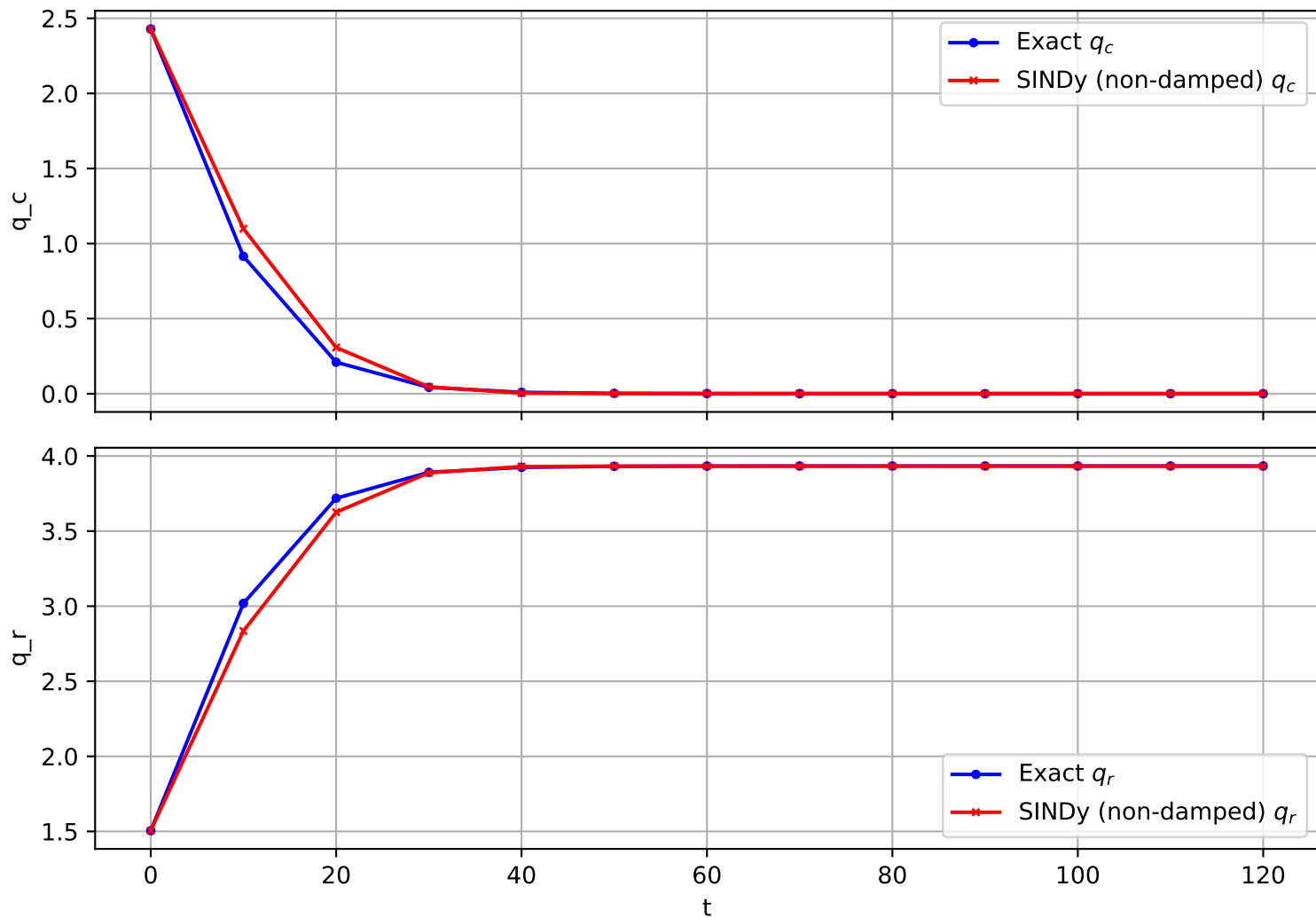
Trajectory 1301 (non-damped)
