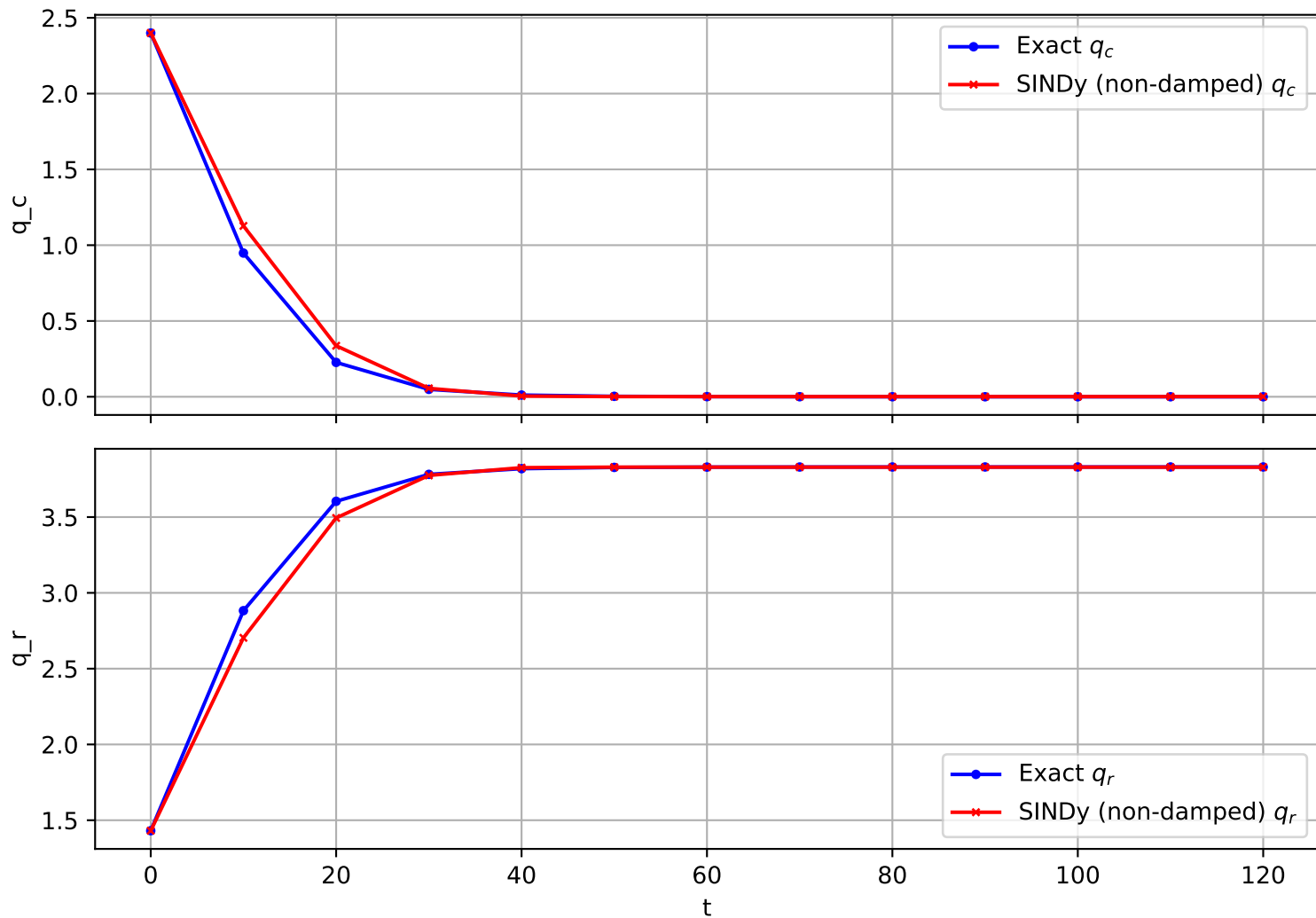
Trajectory 1303 (non-damped)
