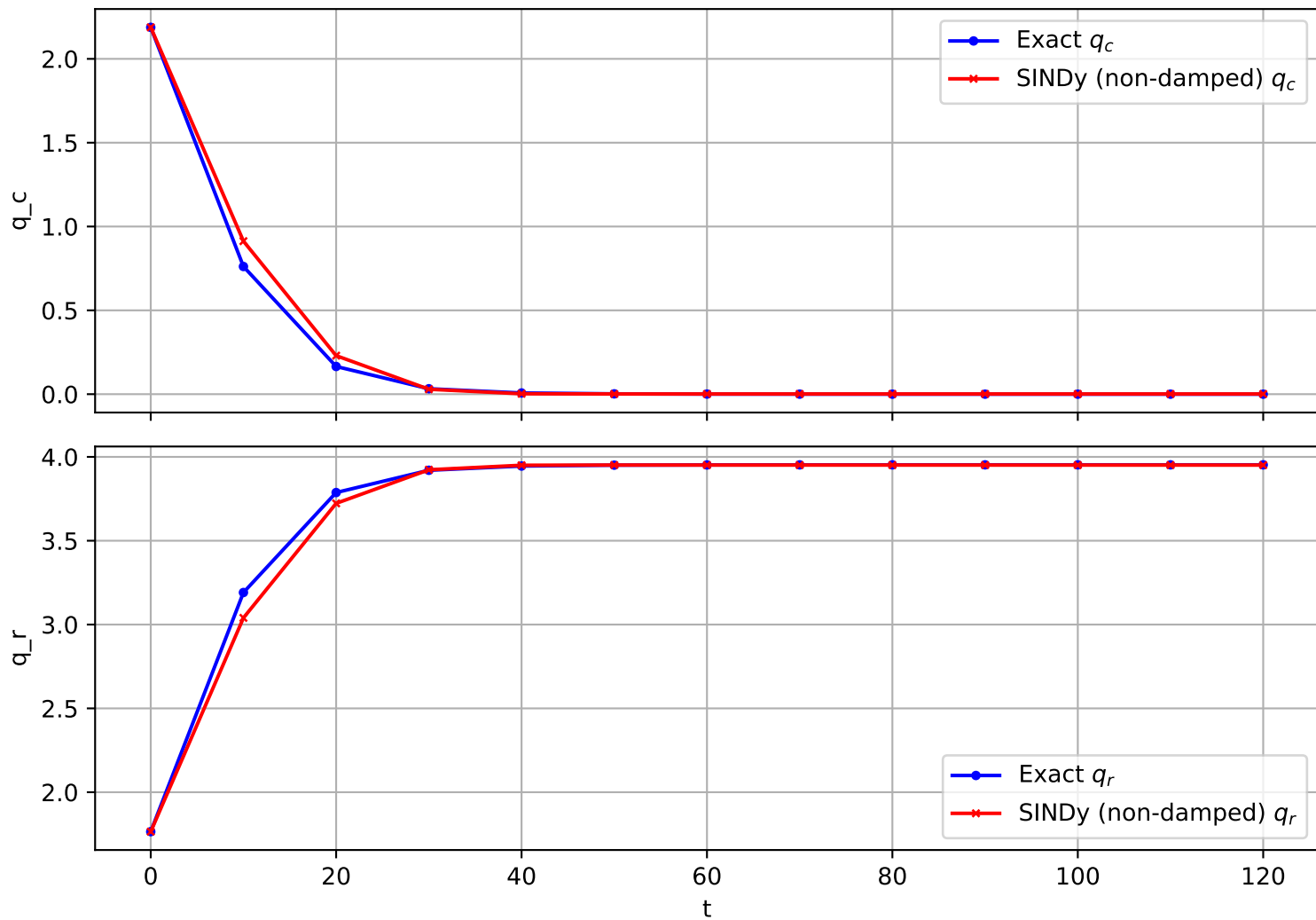
Trajectory 1305 (non-damped)
