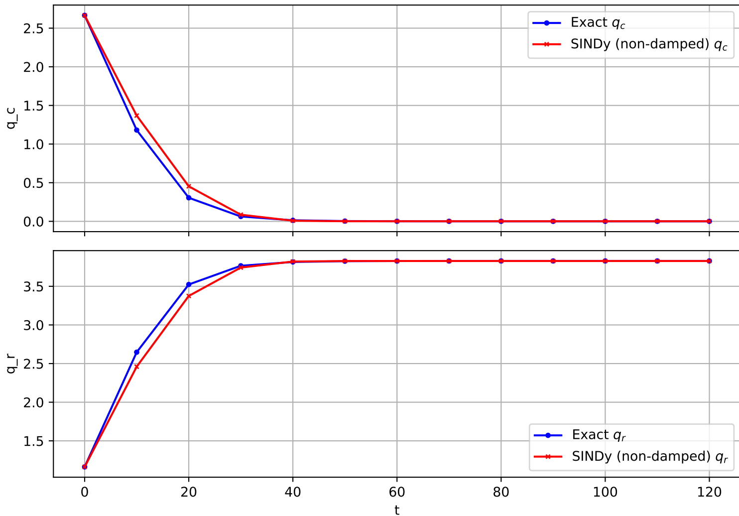
Trajectory 1313 (non-damped)
