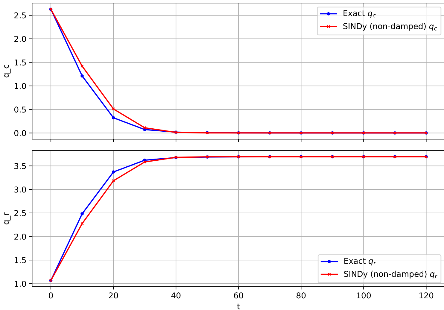
Trajectory 1320 (non-damped)
