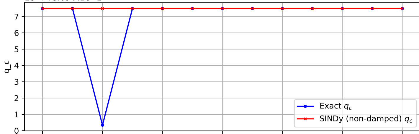
Trajectory 1336 (non-damped)
