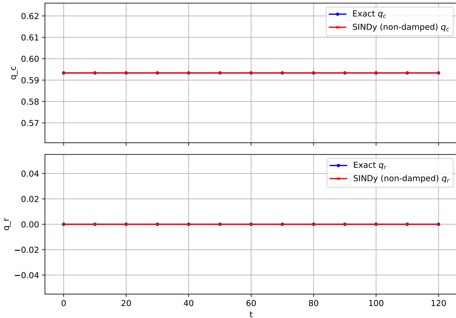
Trajectory 1337 (non-damped)
