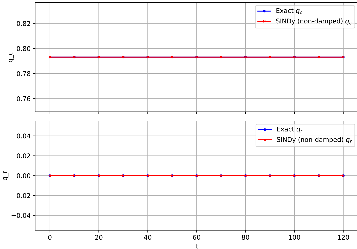
Trajectory 1343 (non-damped)
