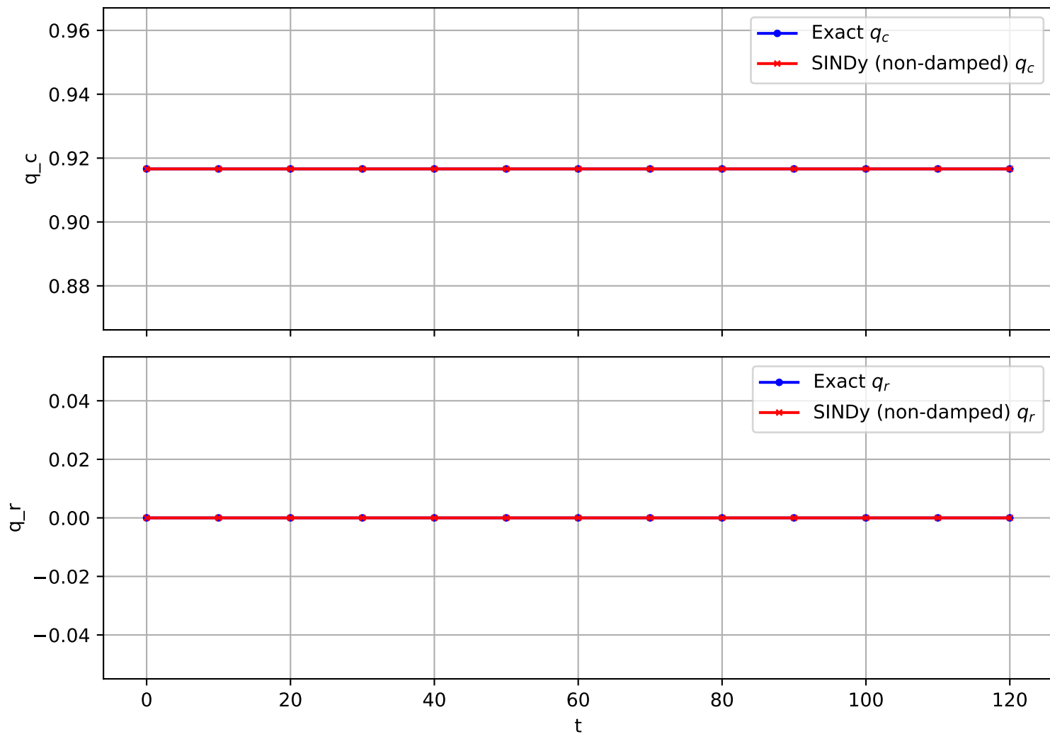
Trajectory 1351 (non-damped)
