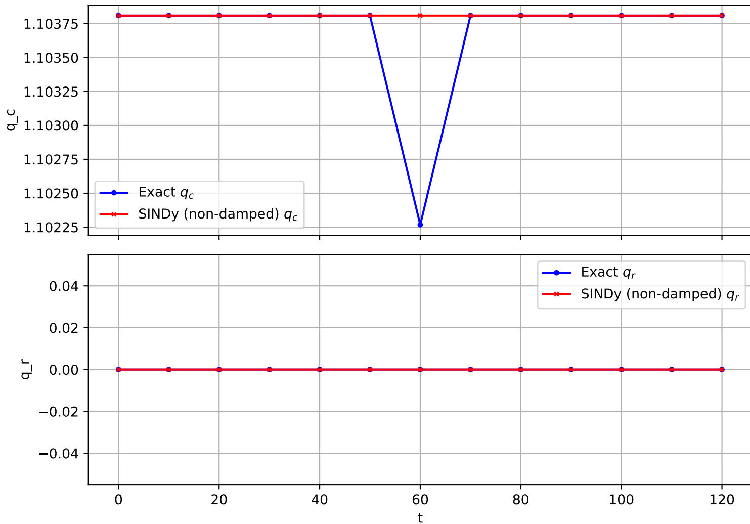
Trajectory 1357 (non-damped)
