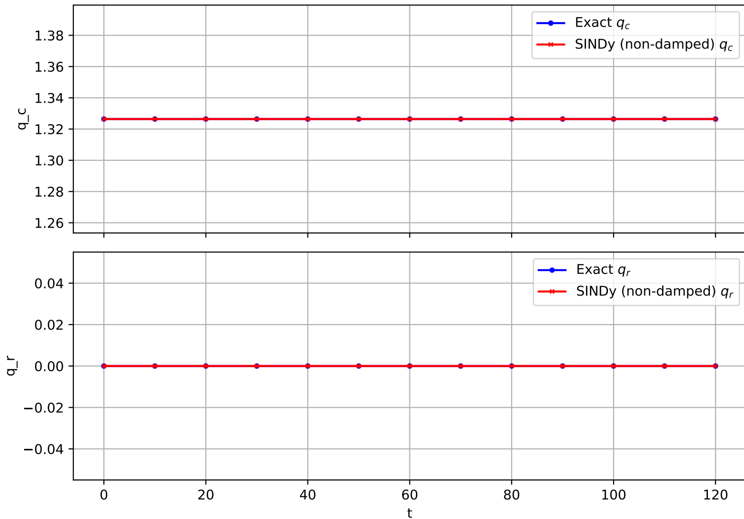
Trajectory 1359 (non-damped)
