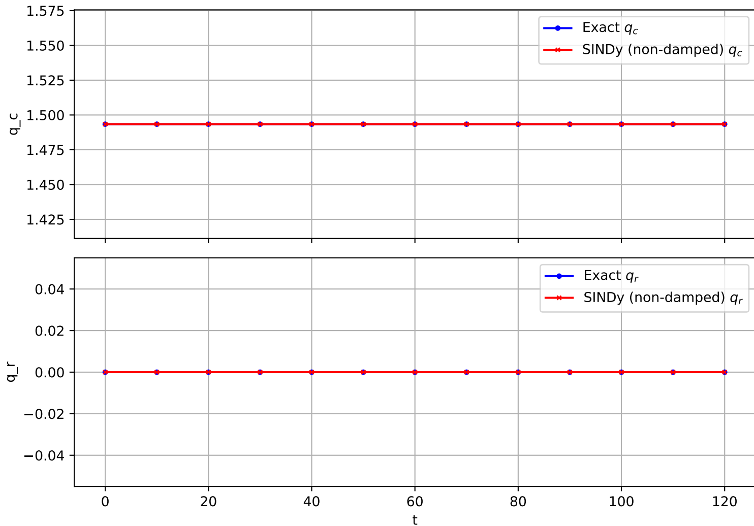
Trajectory 1366 (non-damped)
