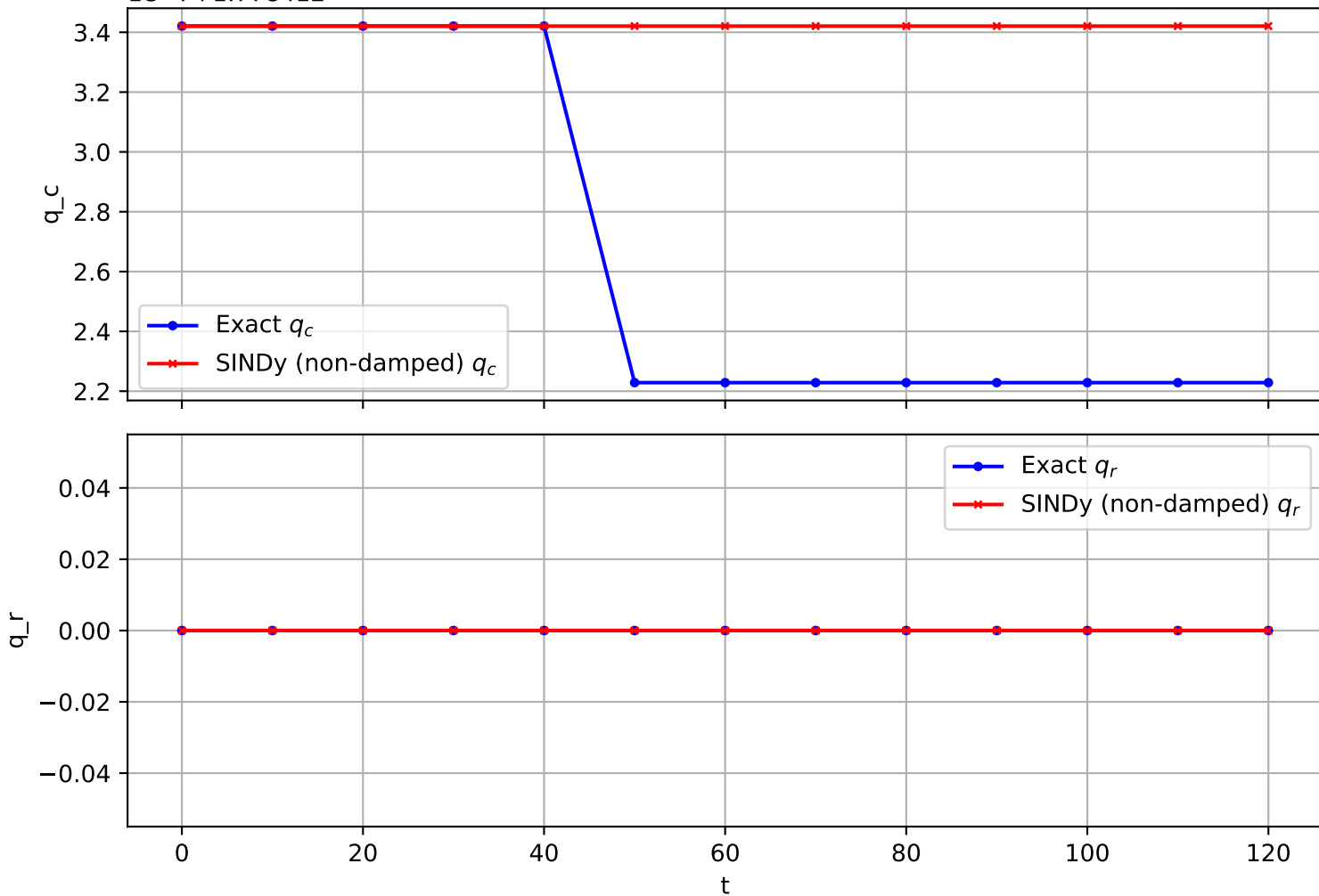
Trajectory 1374 (non-damped)
