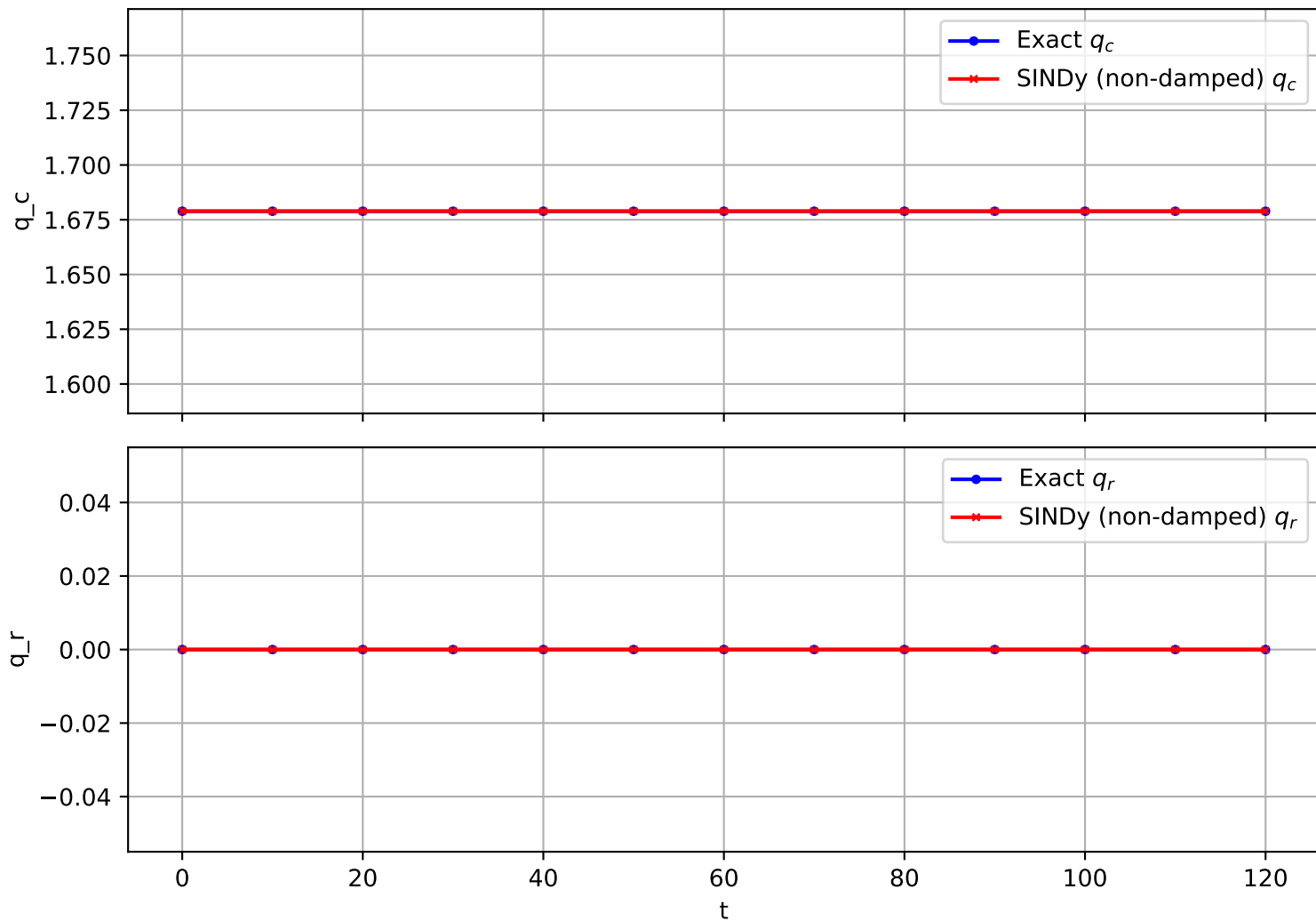
Trajectory 1377 (non-damped)
