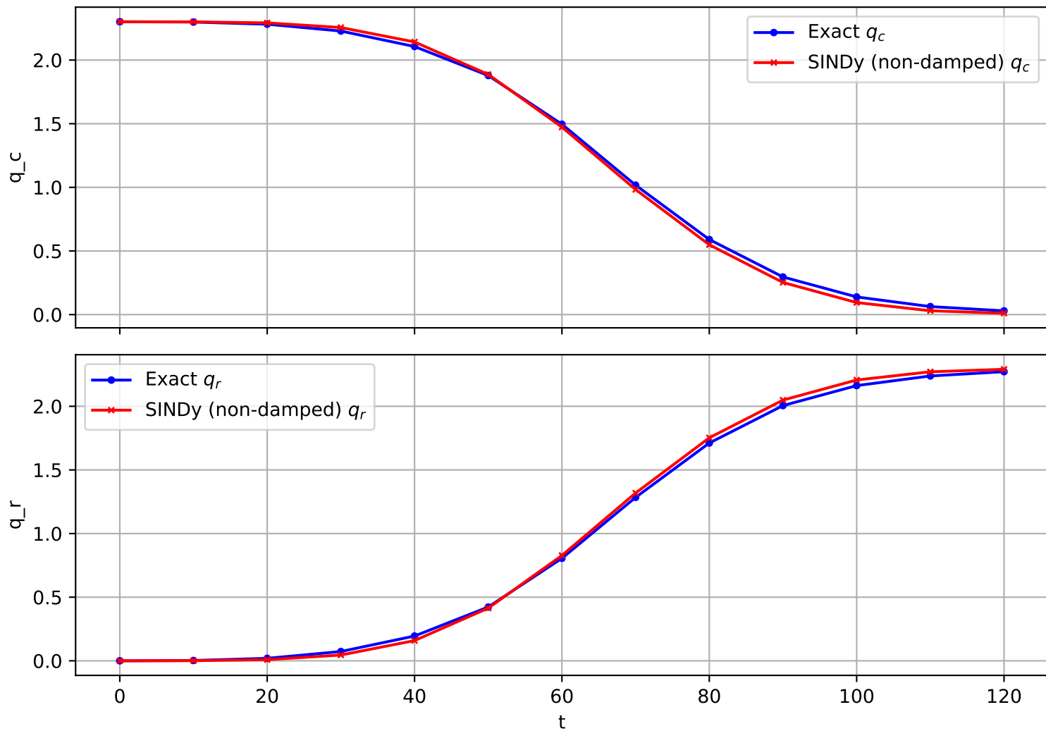
Trajectory 139 (non-damped)
