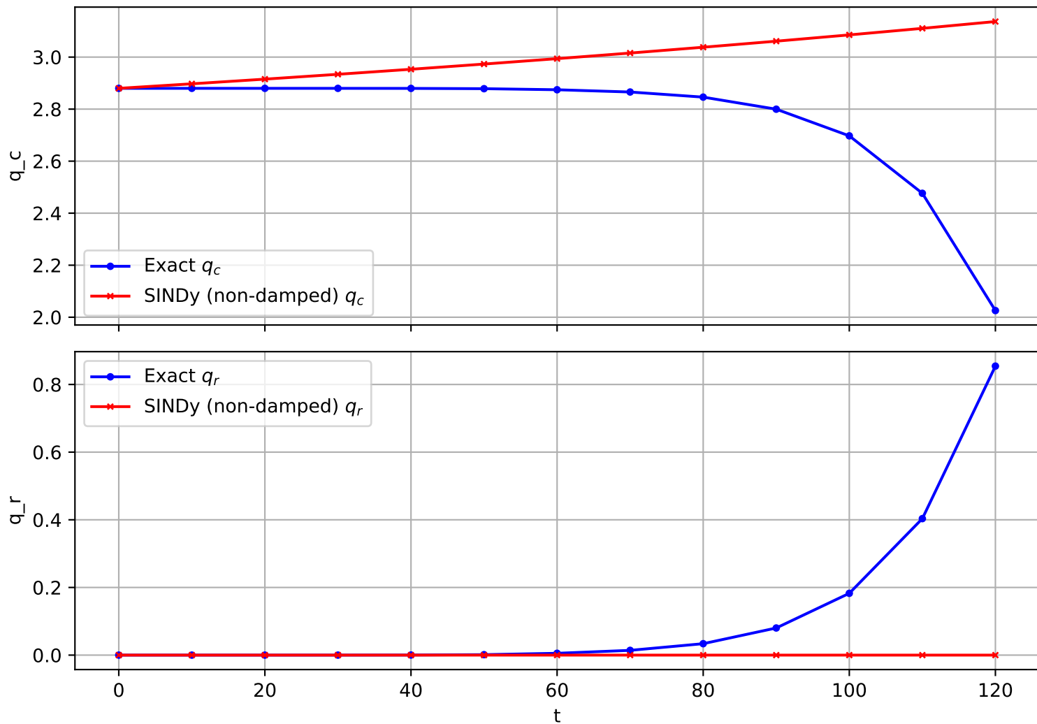
Trajectory 1396 (non-damped)
