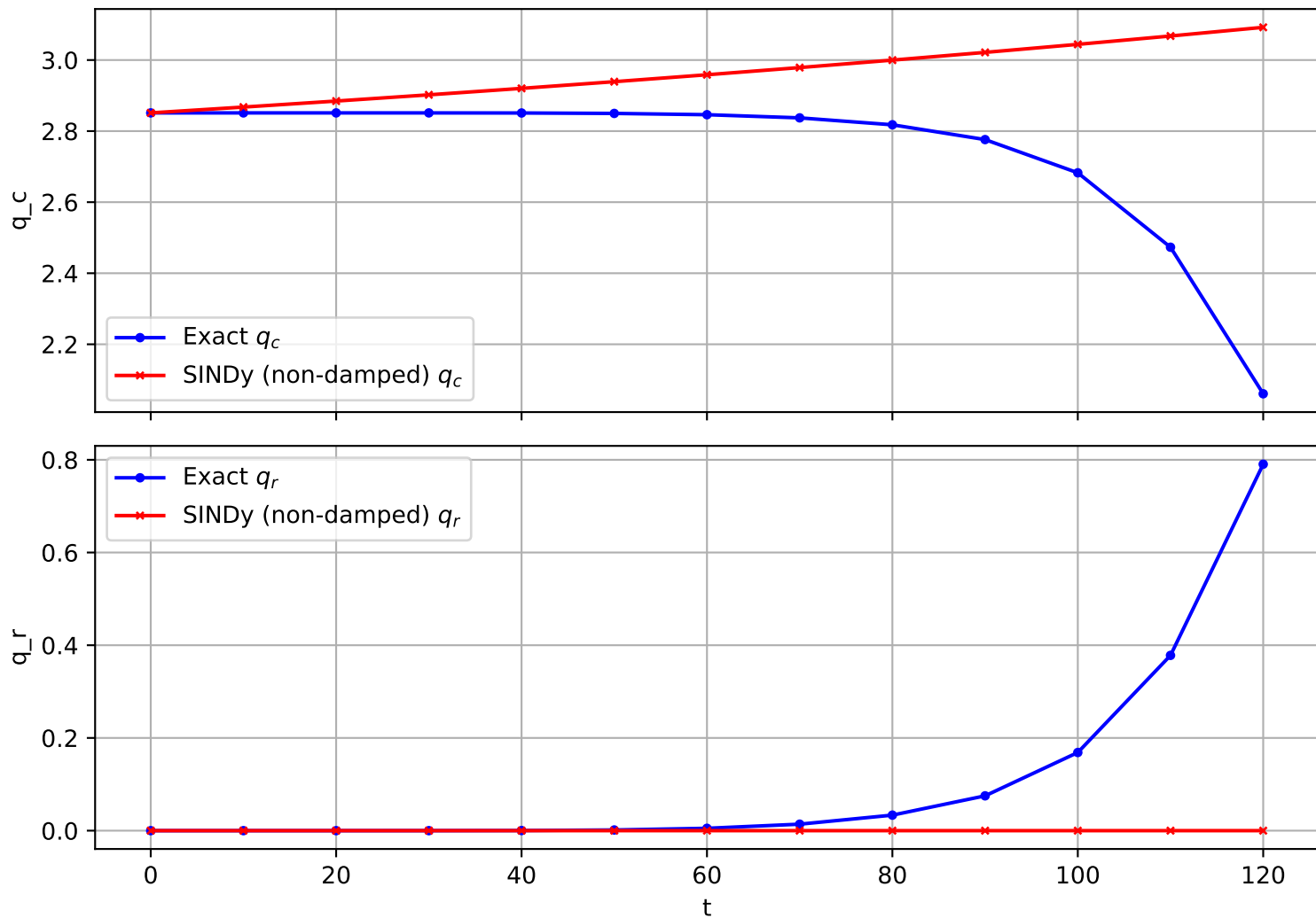
Trajectory 1398 (non-damped)
