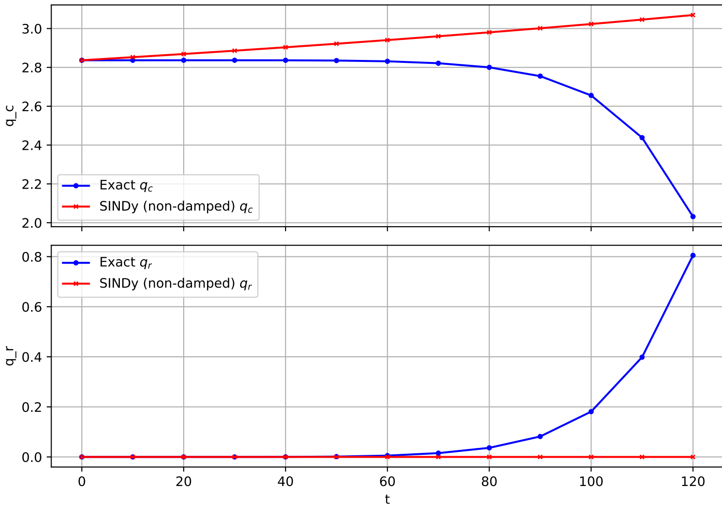
Trajectory 1399 (non-damped)
