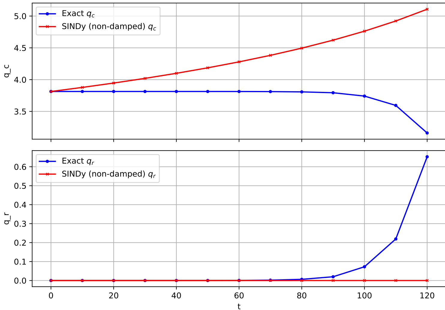
Trajectory 1432 (non-damped)
