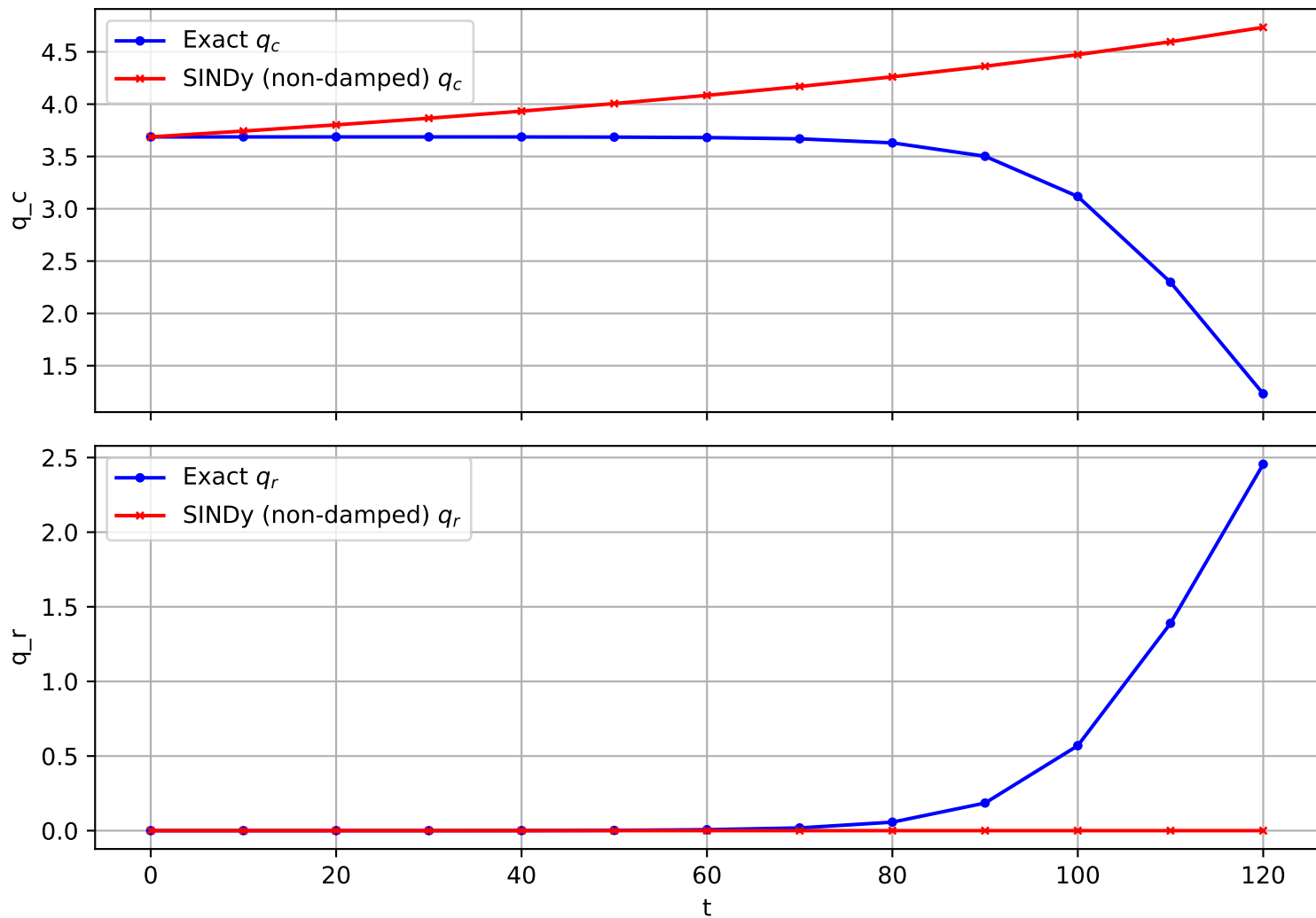
Trajectory 1435 (non-damped)
