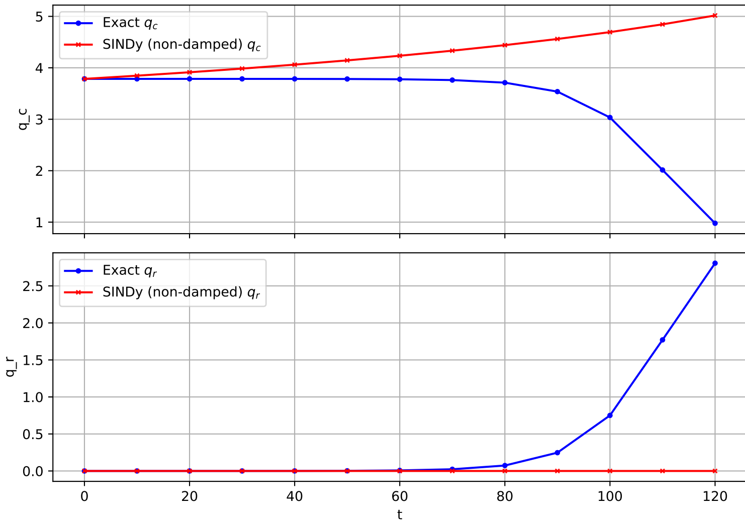
Trajectory 1439 (non-damped)
