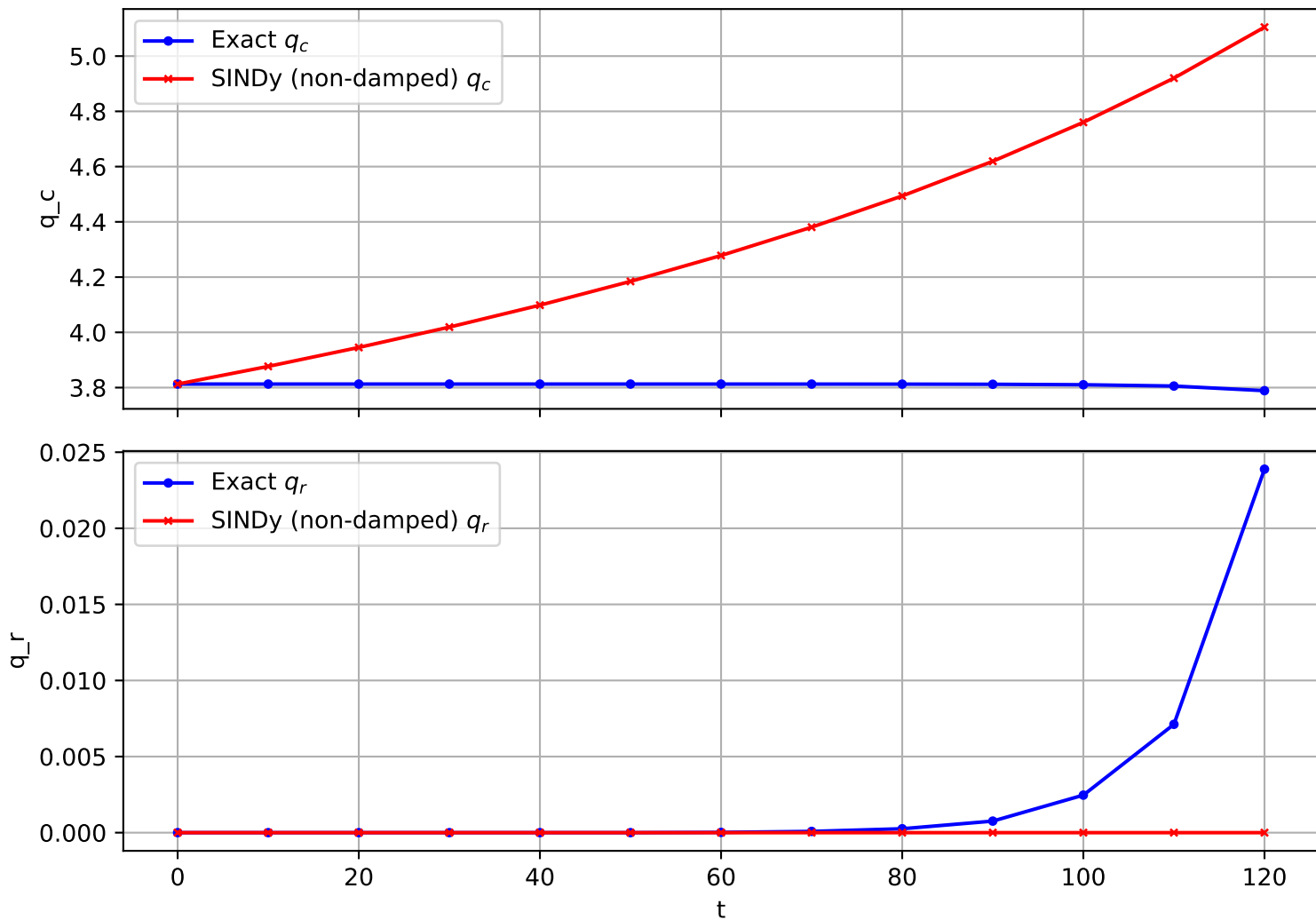
Trajectory 1443 (non-damped)
