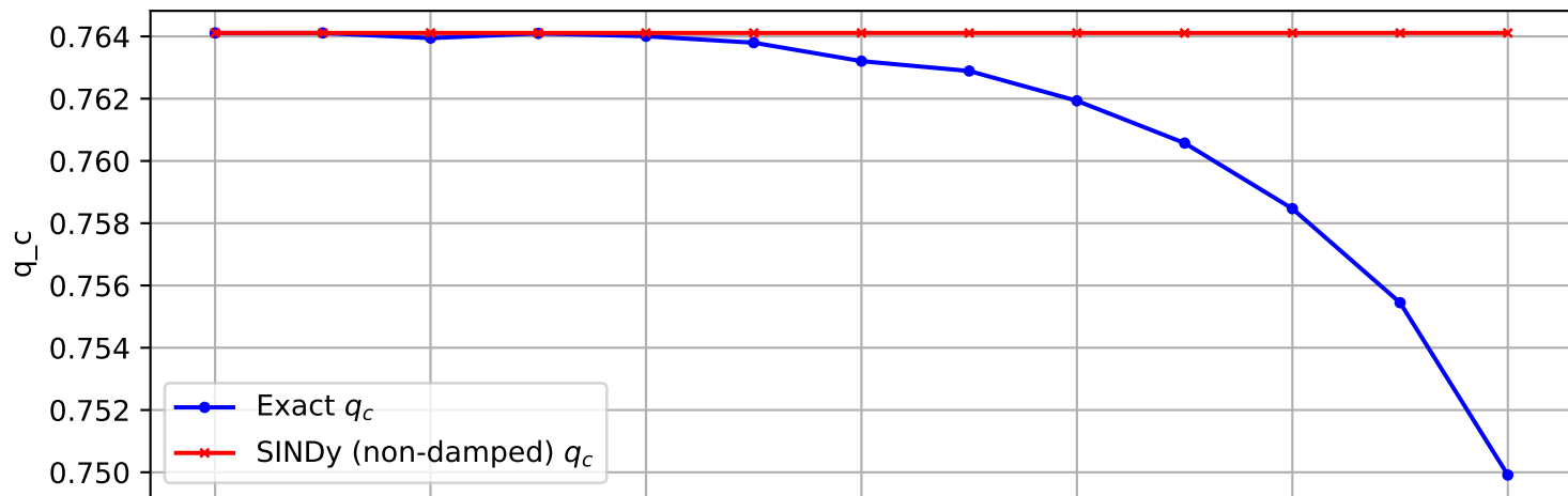
Trajectory 1469 (non-damped)
