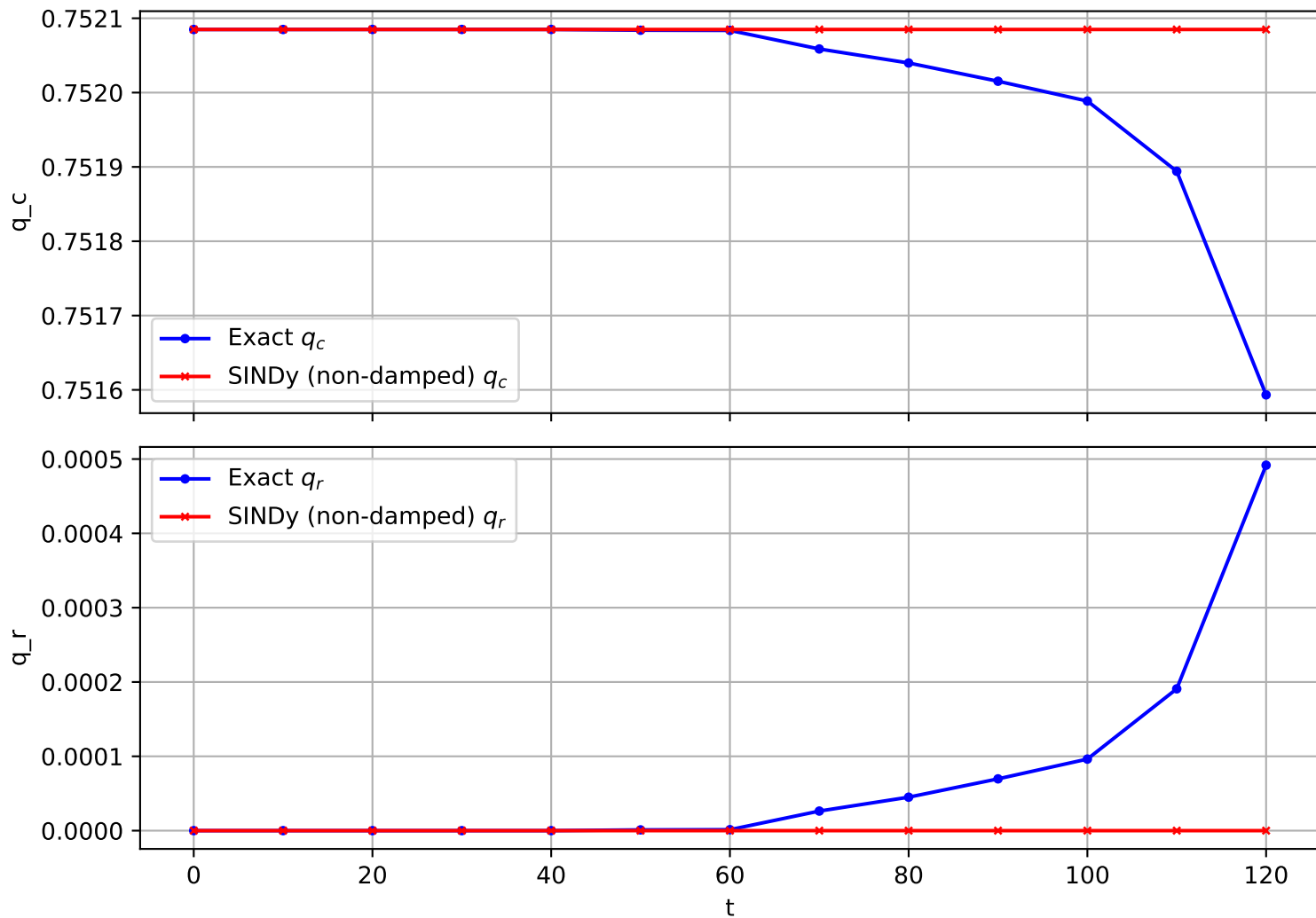
Trajectory 1471 (non-damped)
