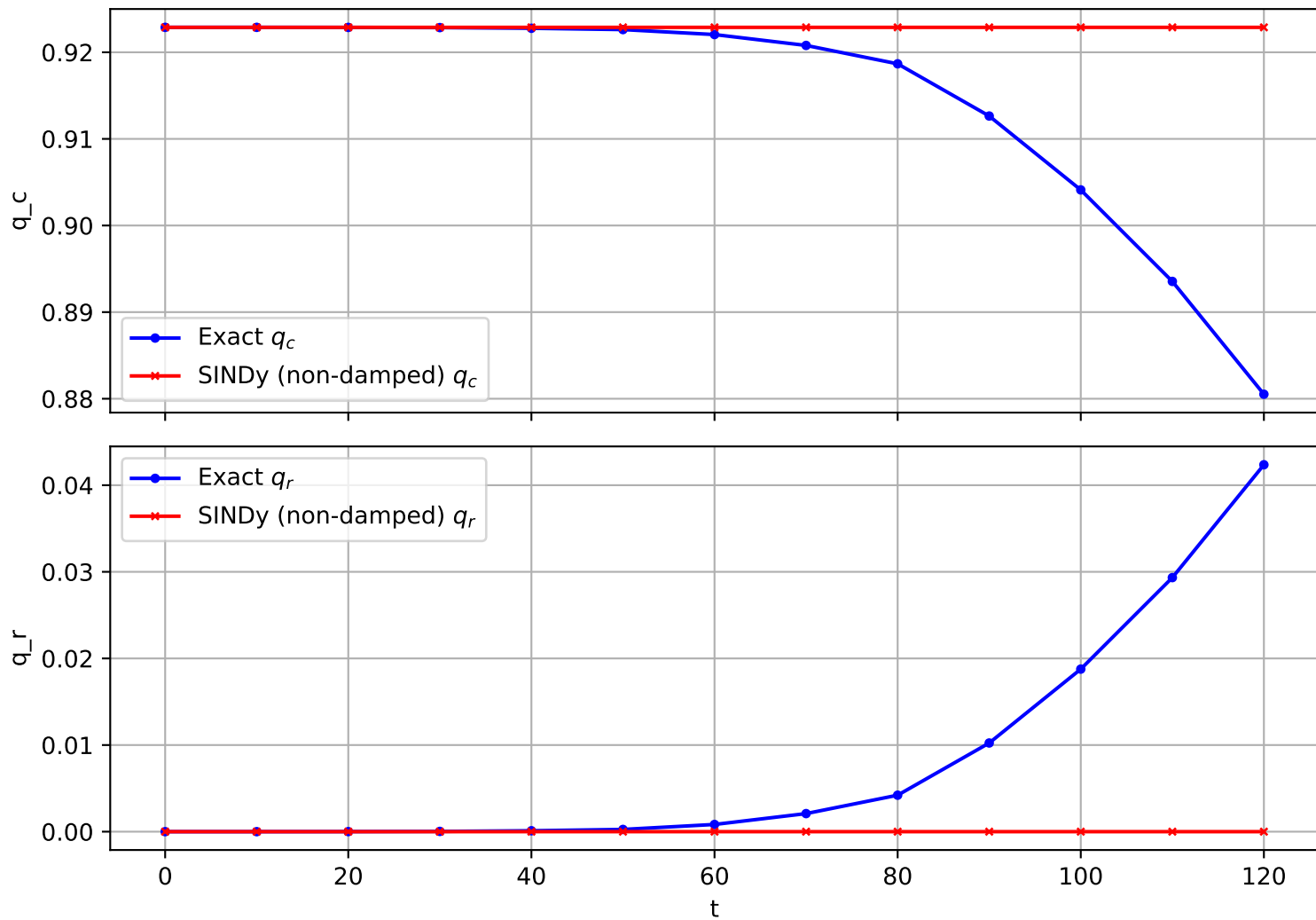
Trajectory 1478 (non-damped)
