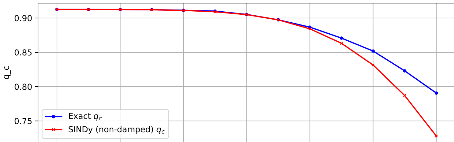
Trajectory 1483 (non-damped)
