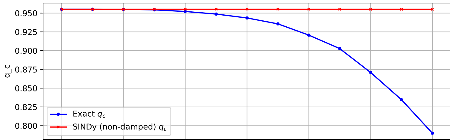
Trajectory 1487 (non-damped)
