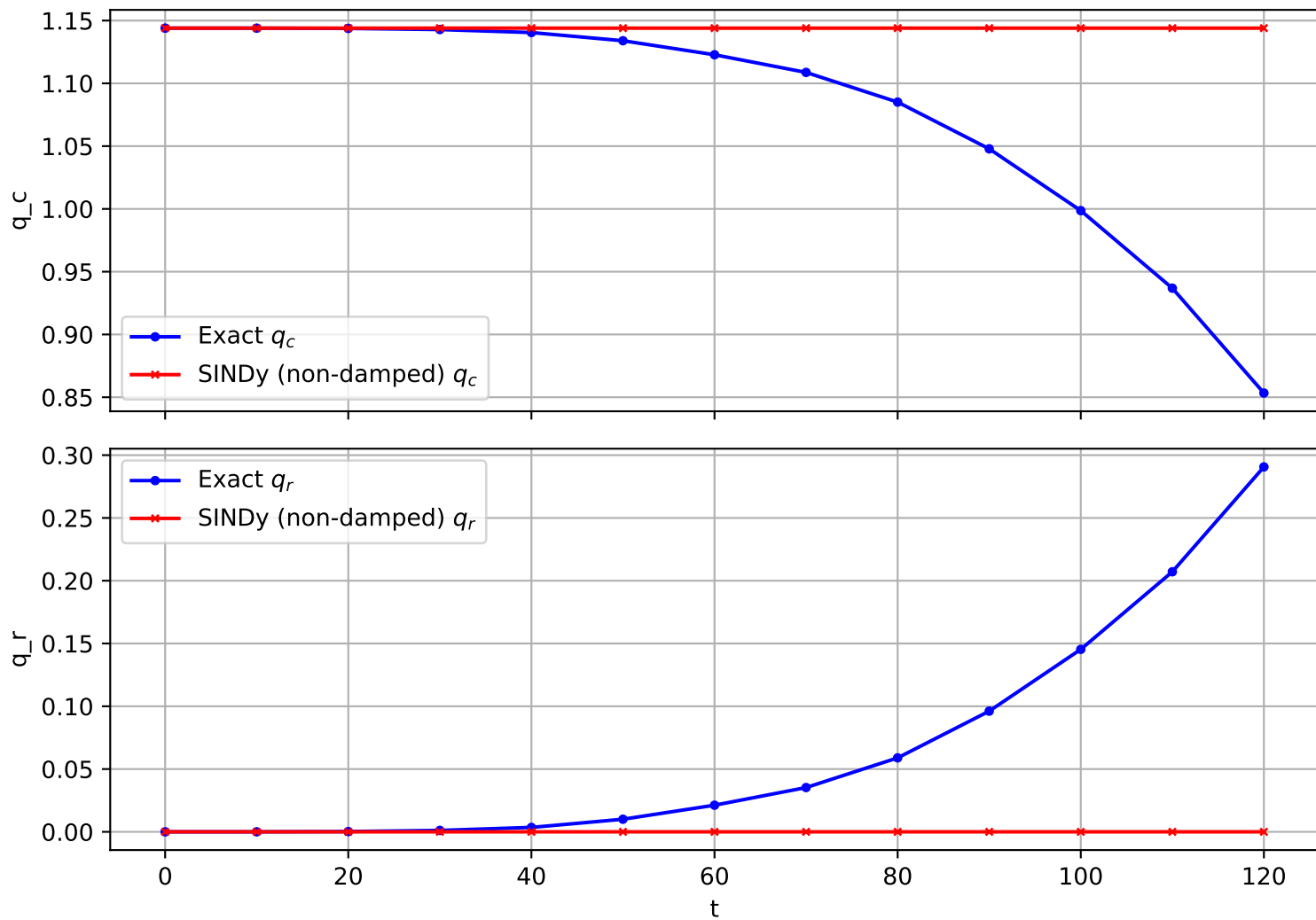
Trajectory 1498 (non-damped)
