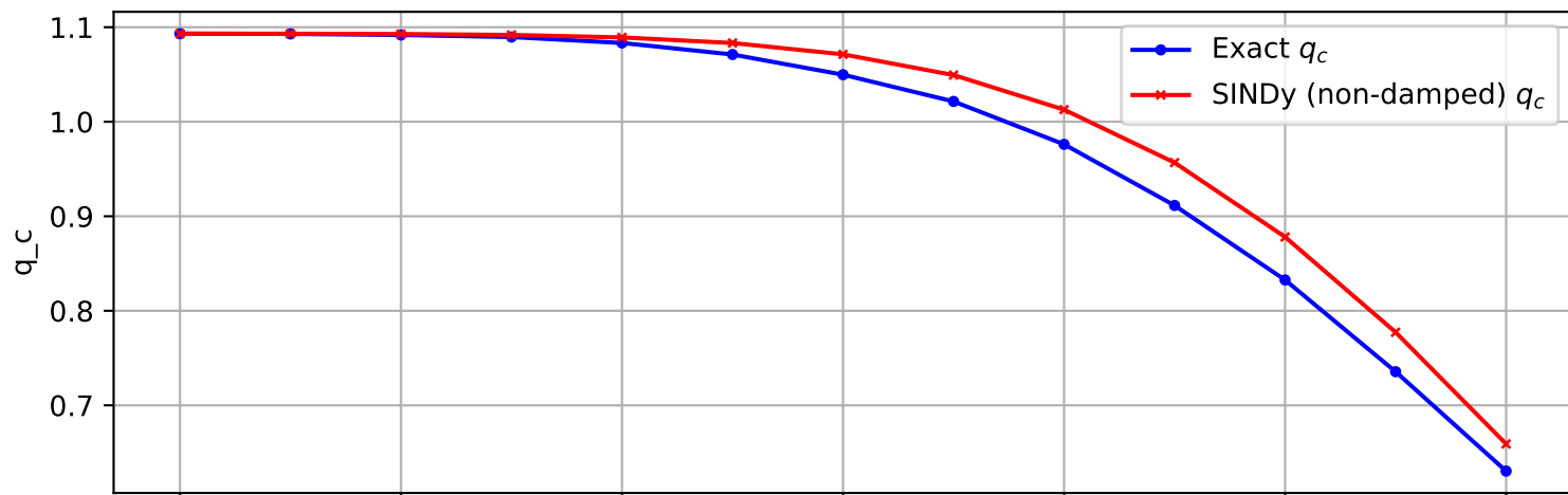
Trajectory 1505 (non-damped)
