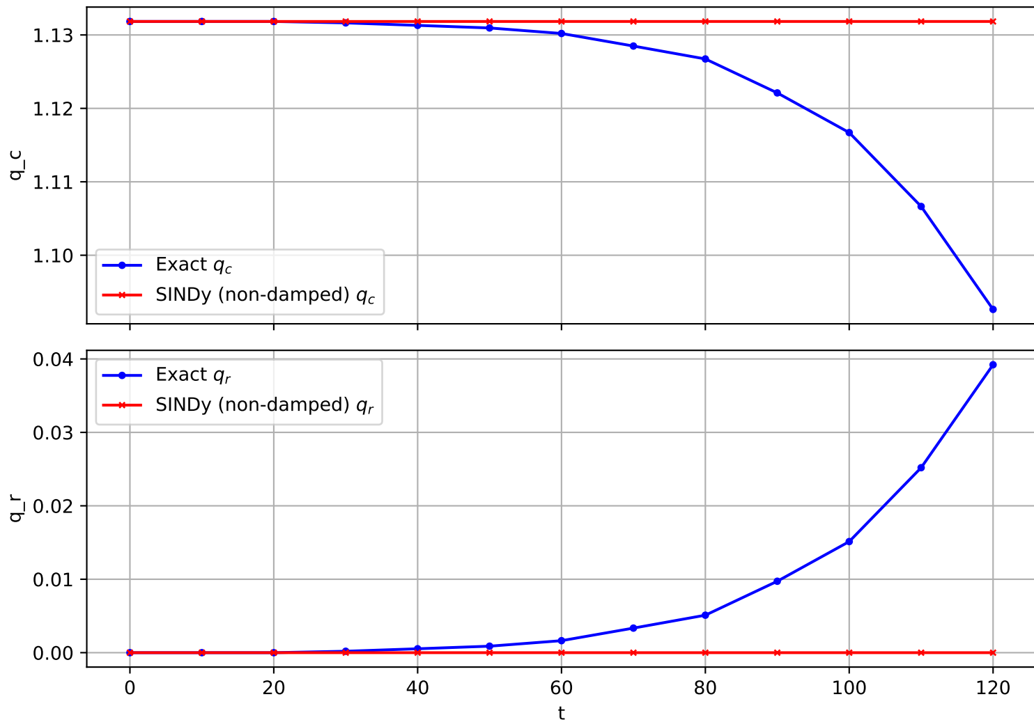
Trajectory 1520 (non-damped)
