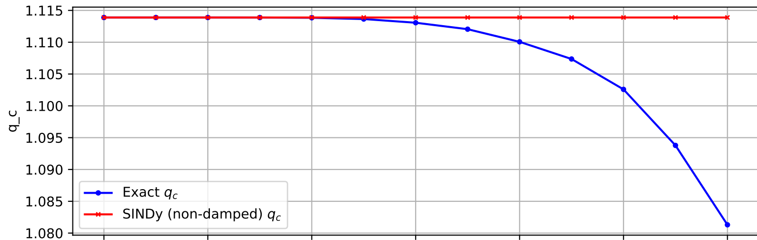
Trajectory 1521 (non-damped)
