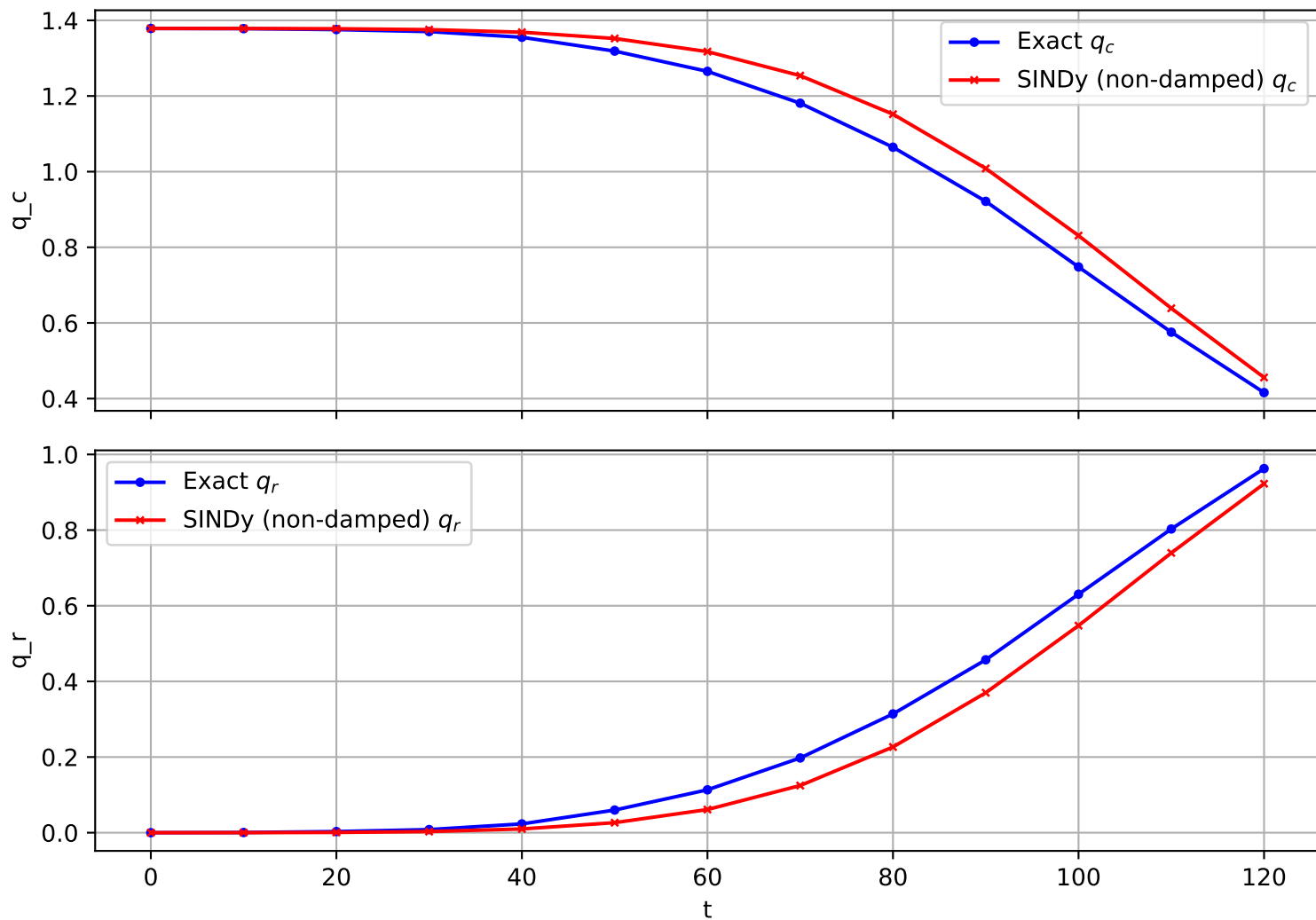
Trajectory 1527 (non-damped)
