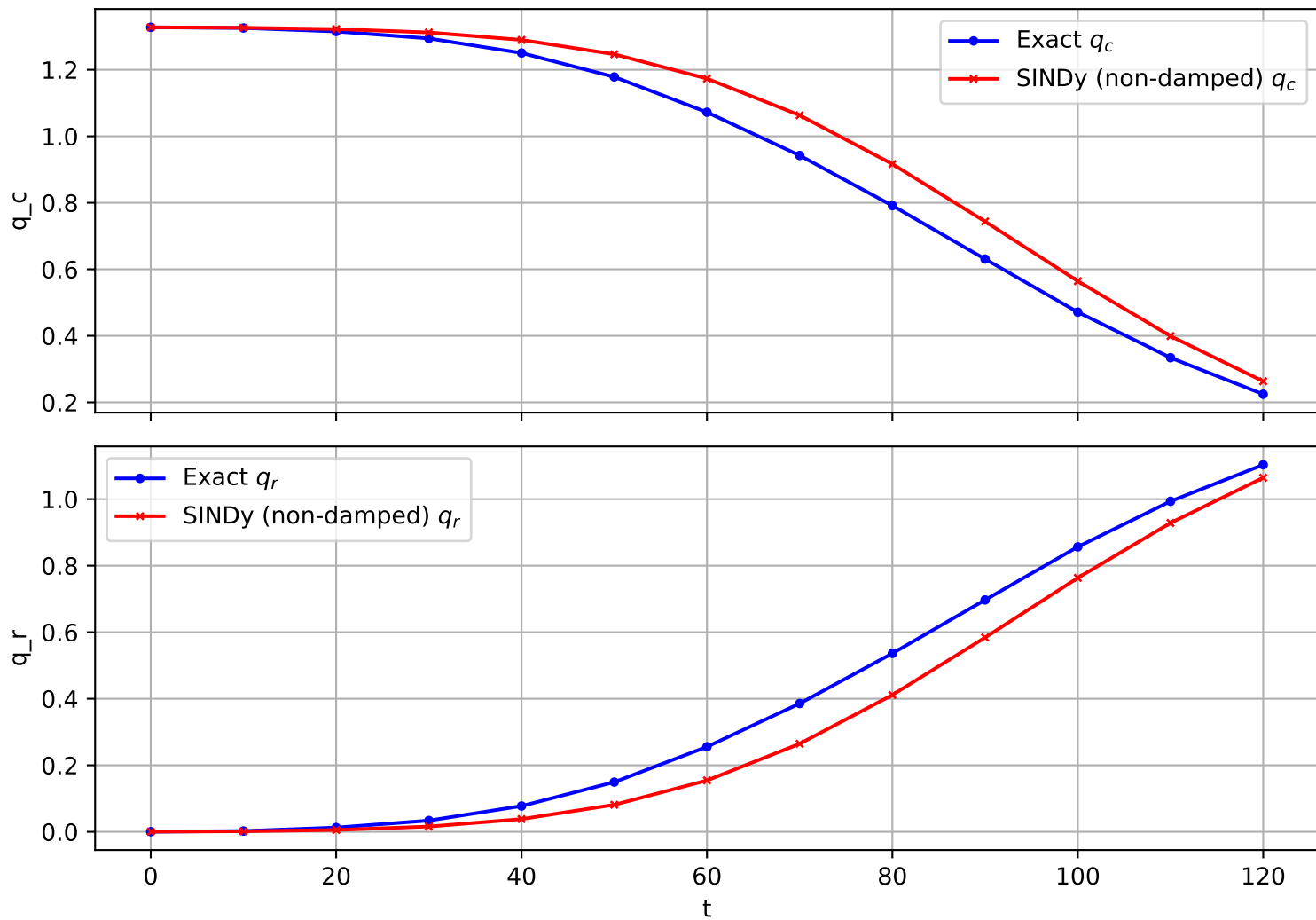
Trajectory 1533 (non-damped)
