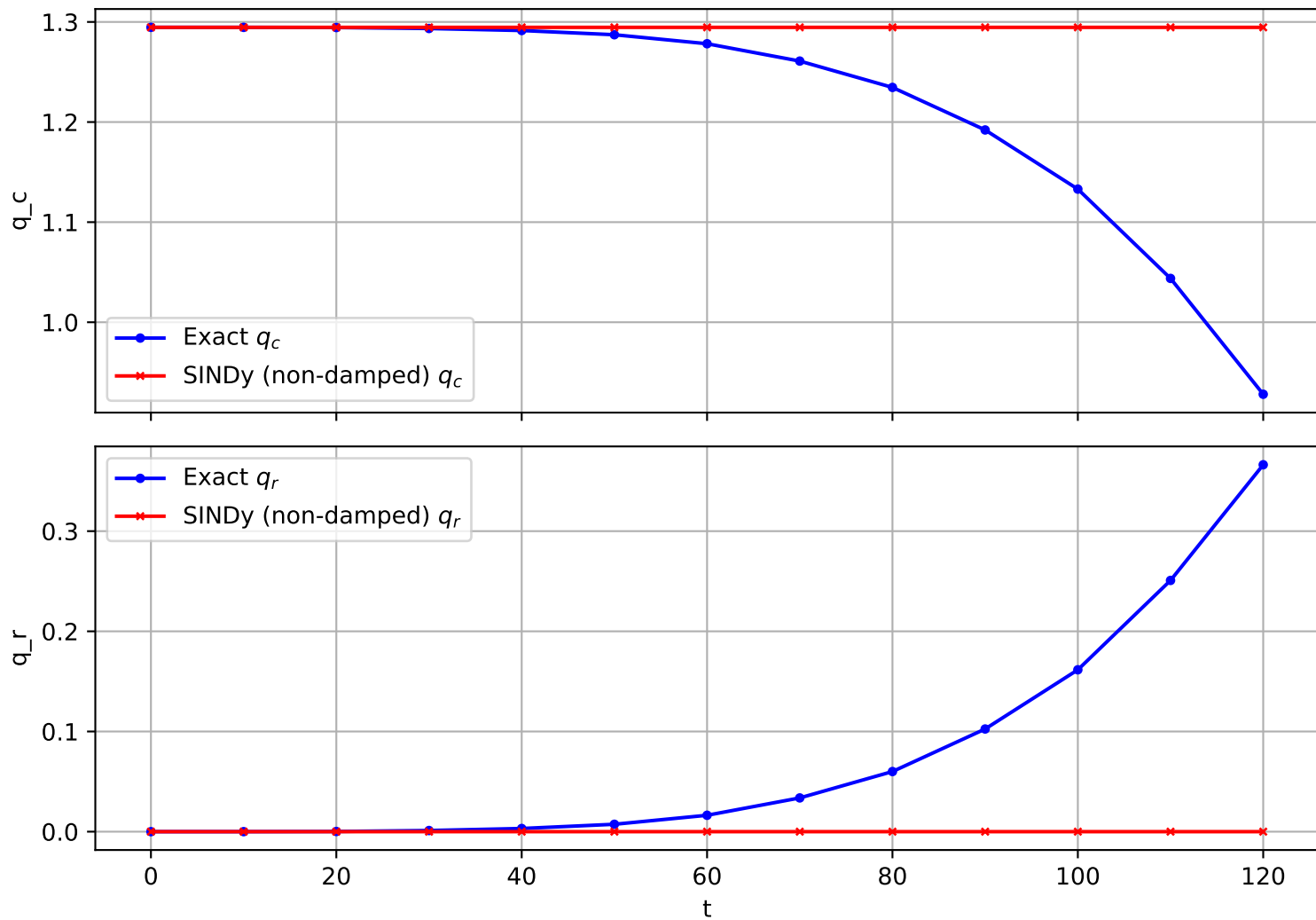
Trajectory 1537 (non-damped)
