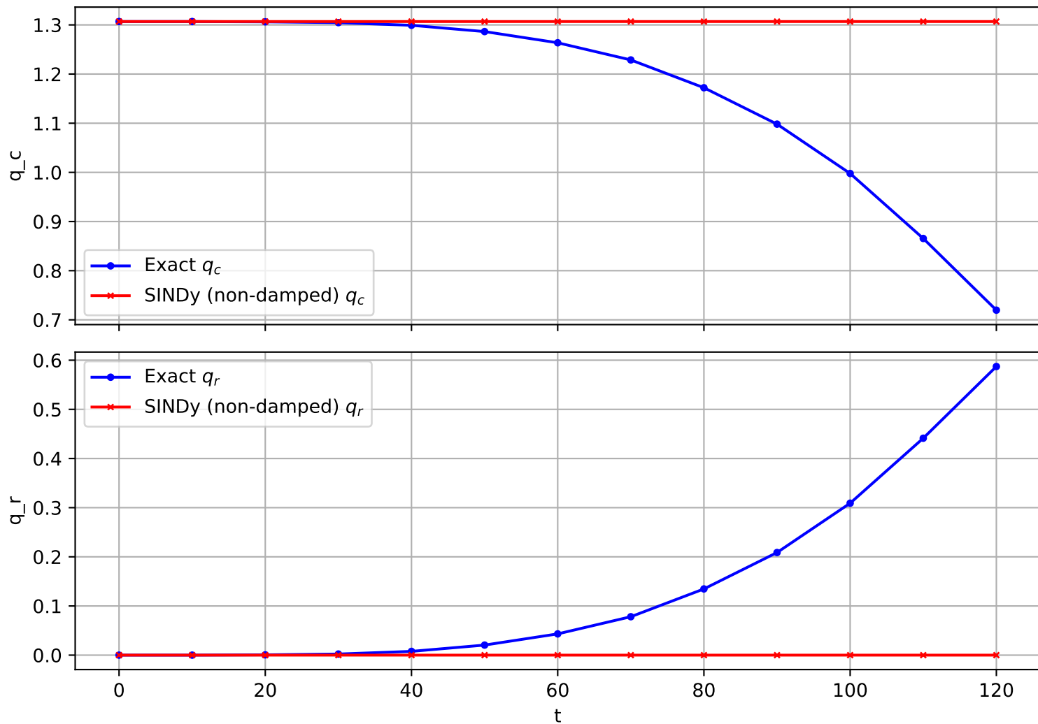
Trajectory 1541 (non-damped)
