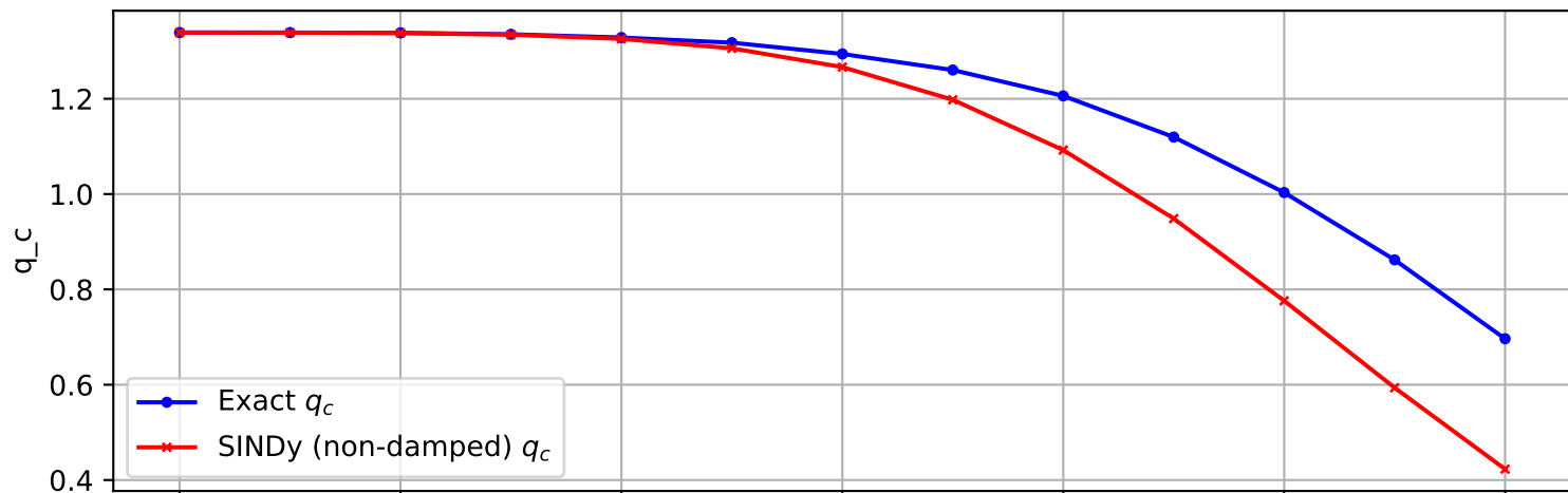
Trajectory 1543 (non-damped)
