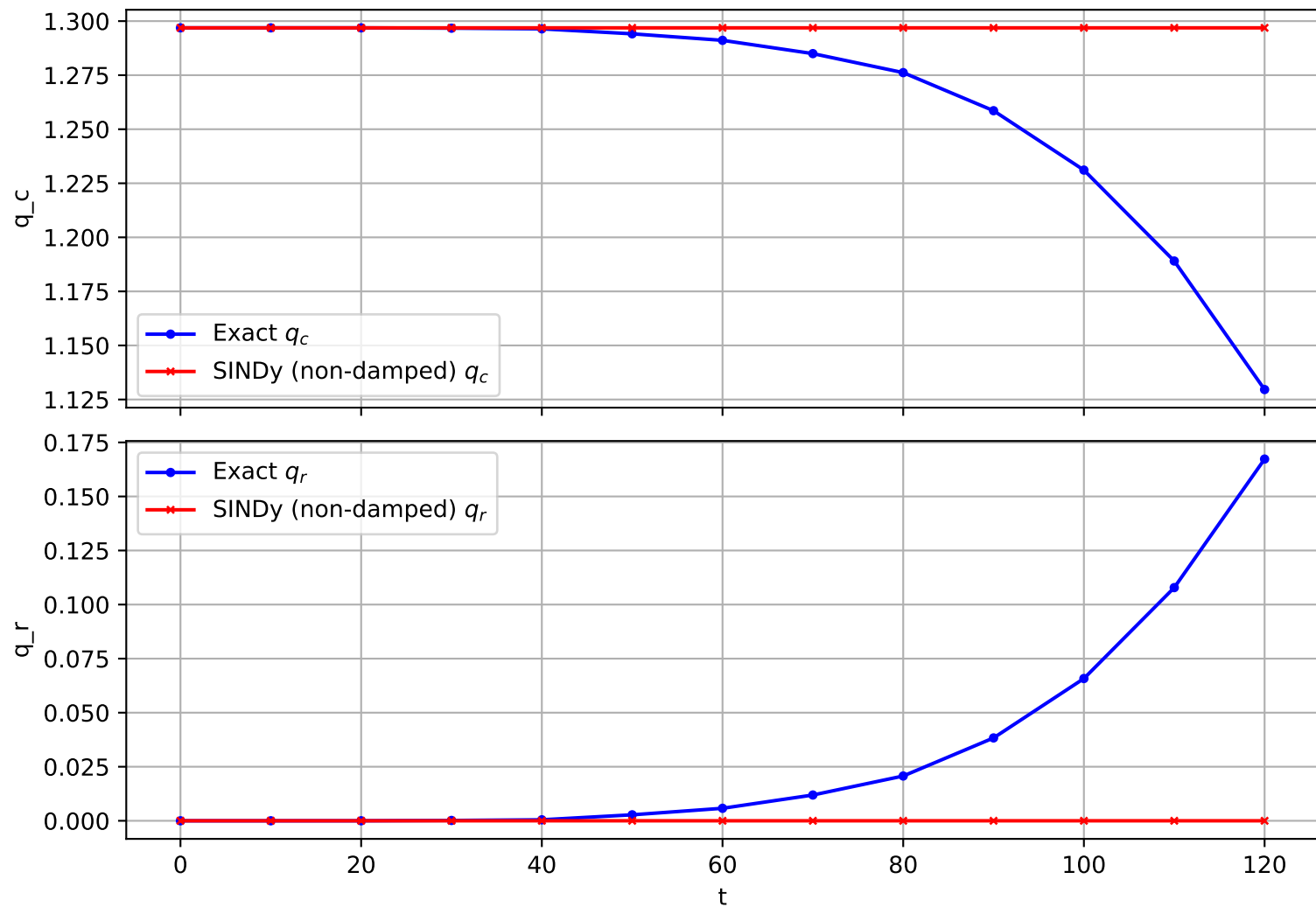
Trajectory 1545 (non-damped)
