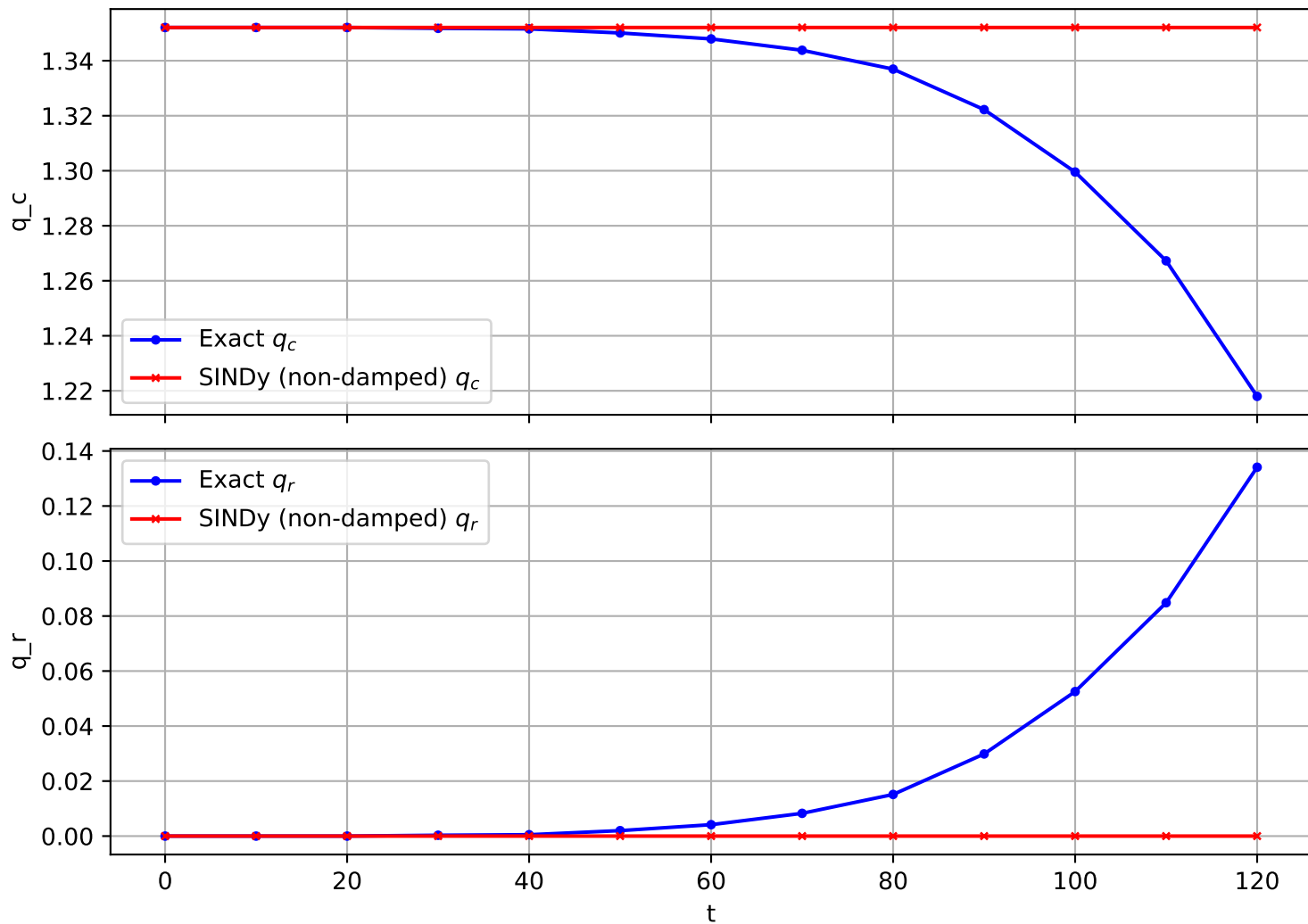
Trajectory 1555 (non-damped)
