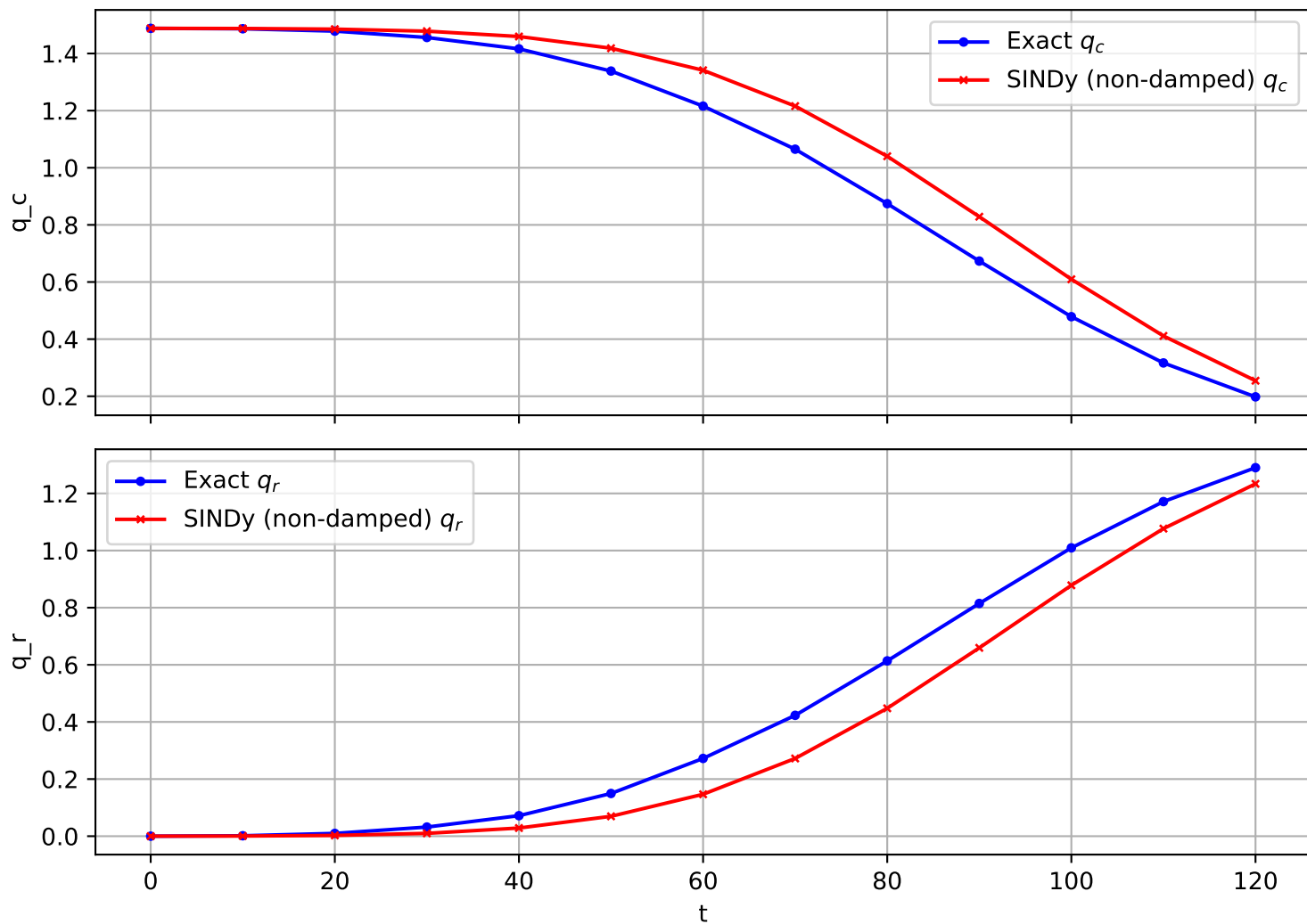
Trajectory 1561 (non-damped)
