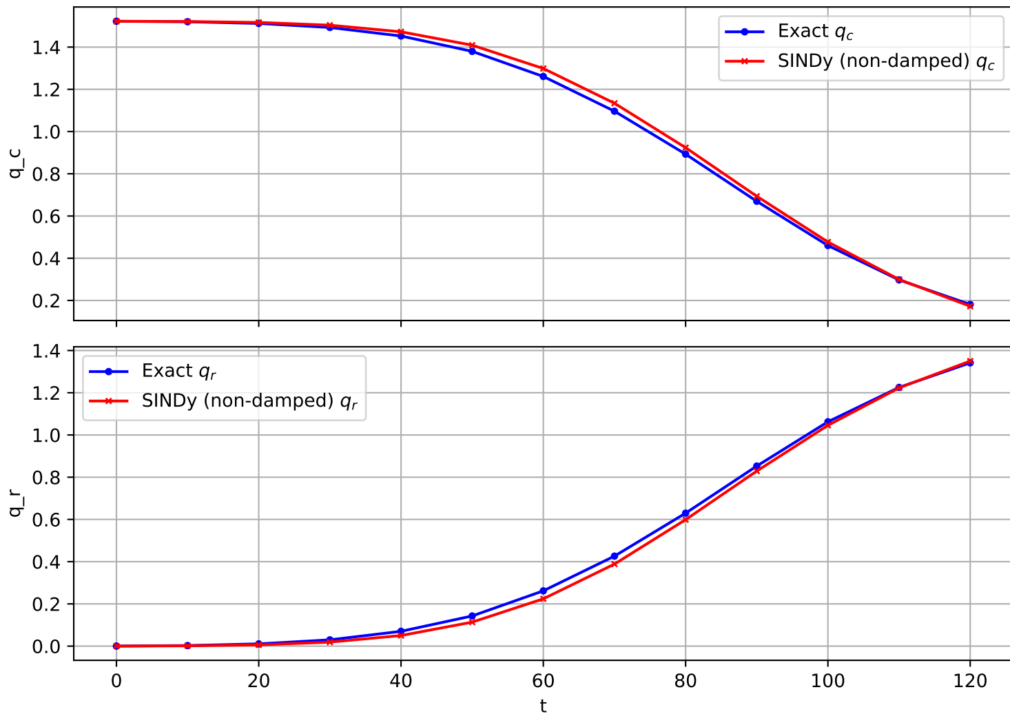
Trajectory 1563 (non-damped)
