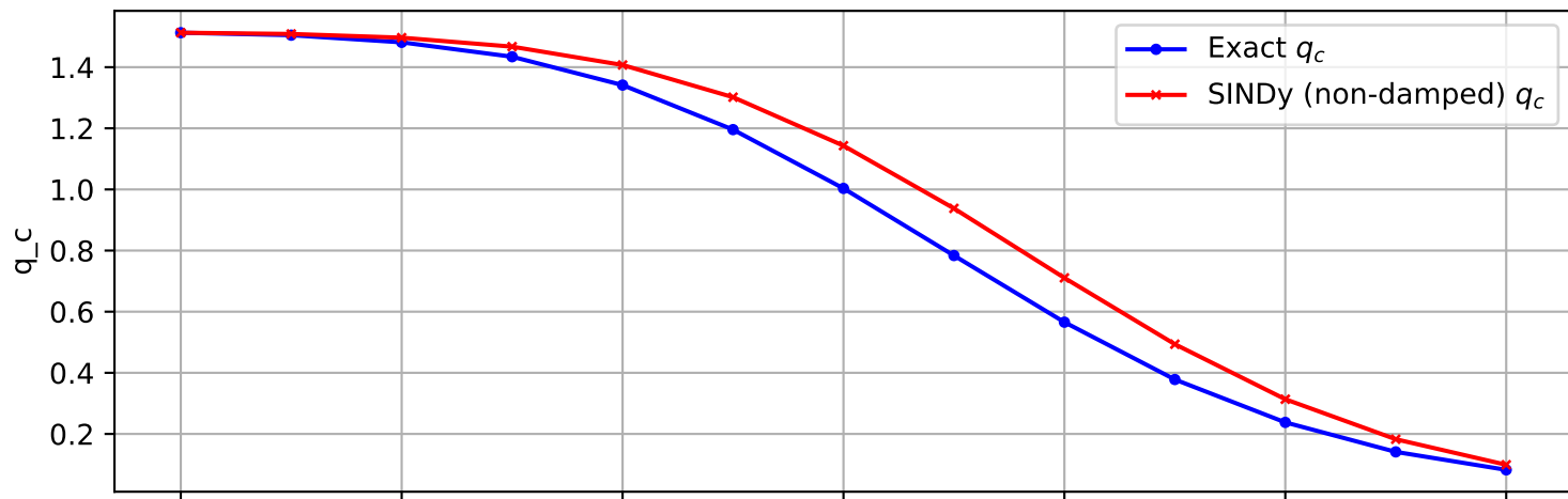
Trajectory 1568 (non-damped)
