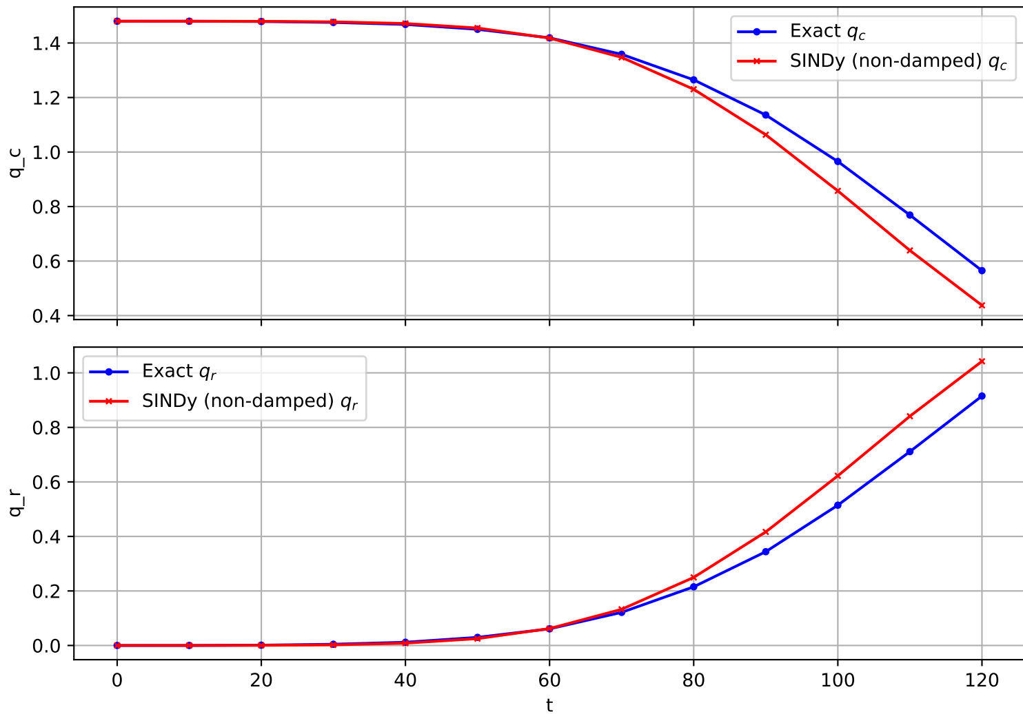
Trajectory 1571 (non-damped)
