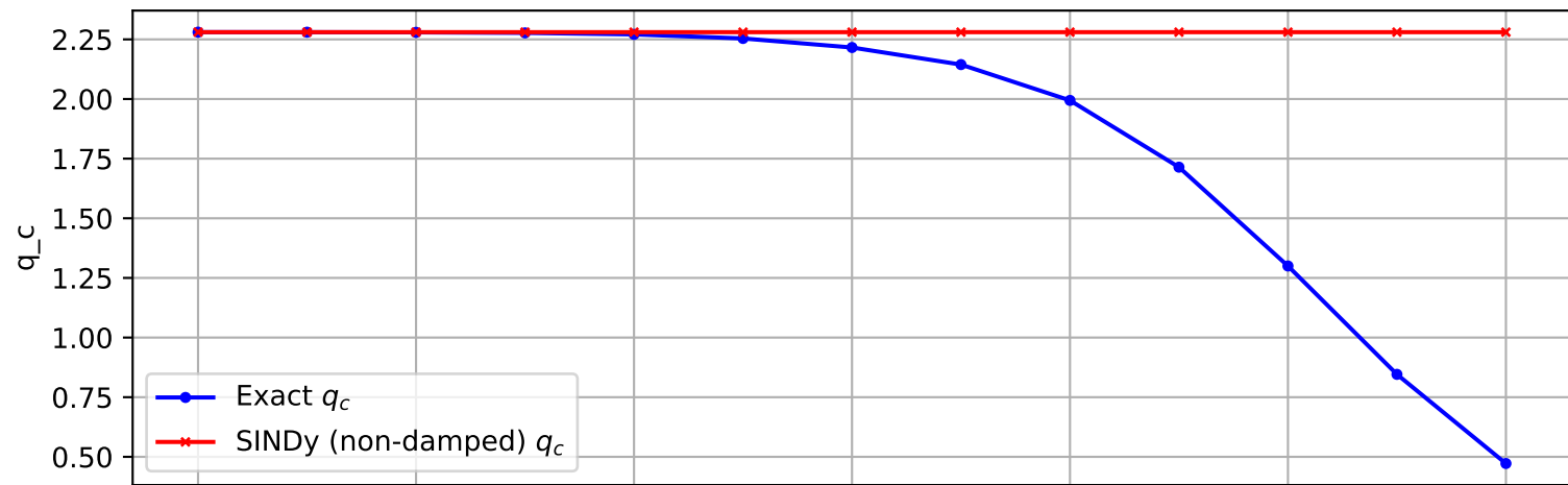
Trajectory 158 (non-damped)
