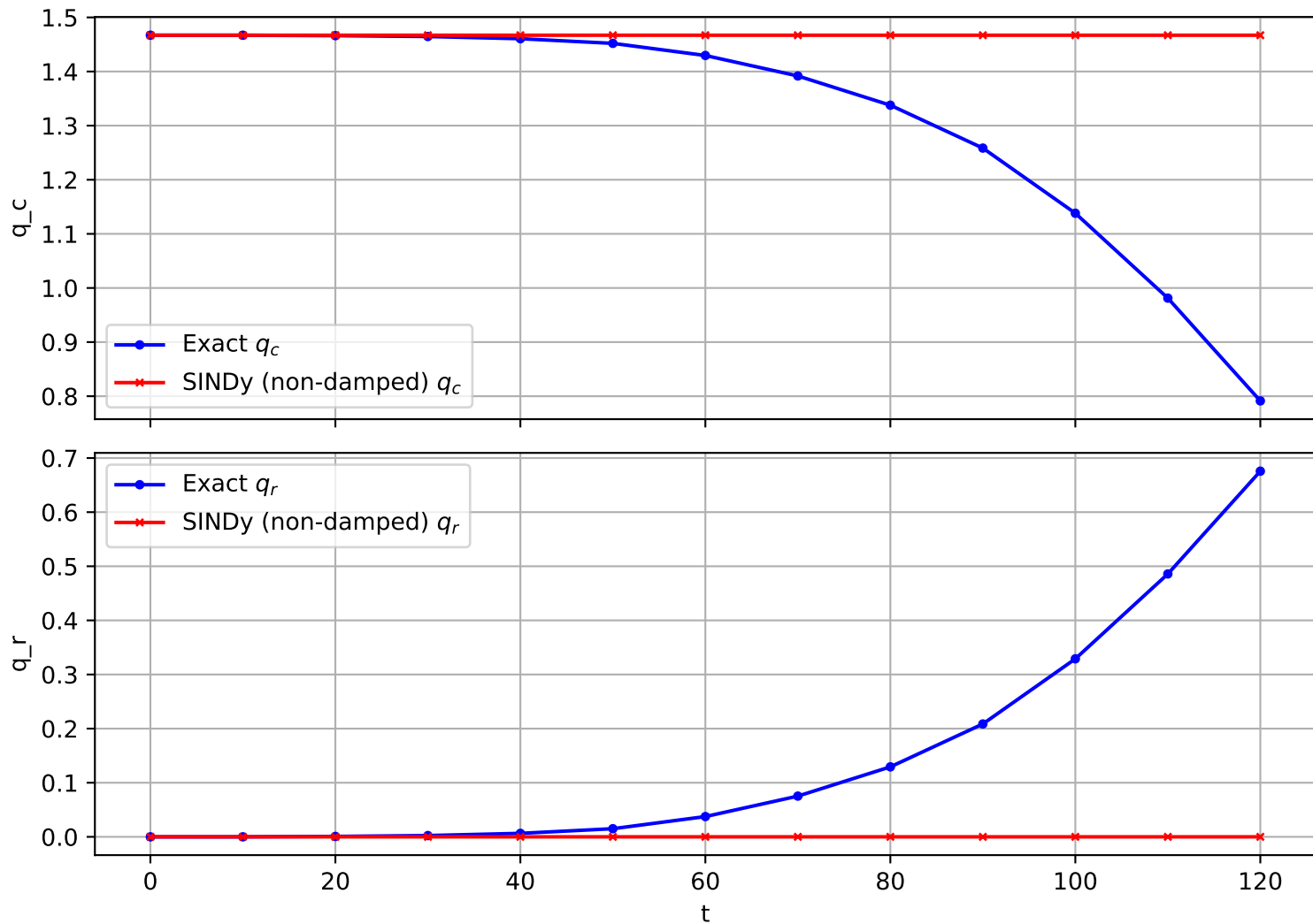
Trajectory 1581 (non-damped)
