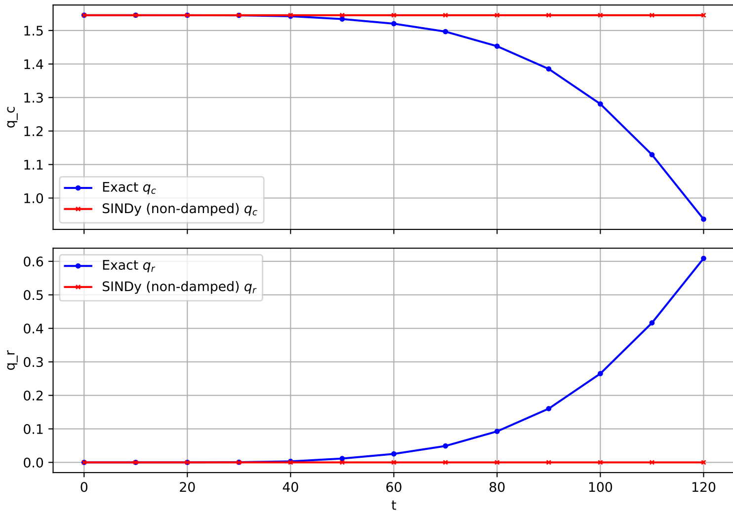
Trajectory 1590 (non-damped)
